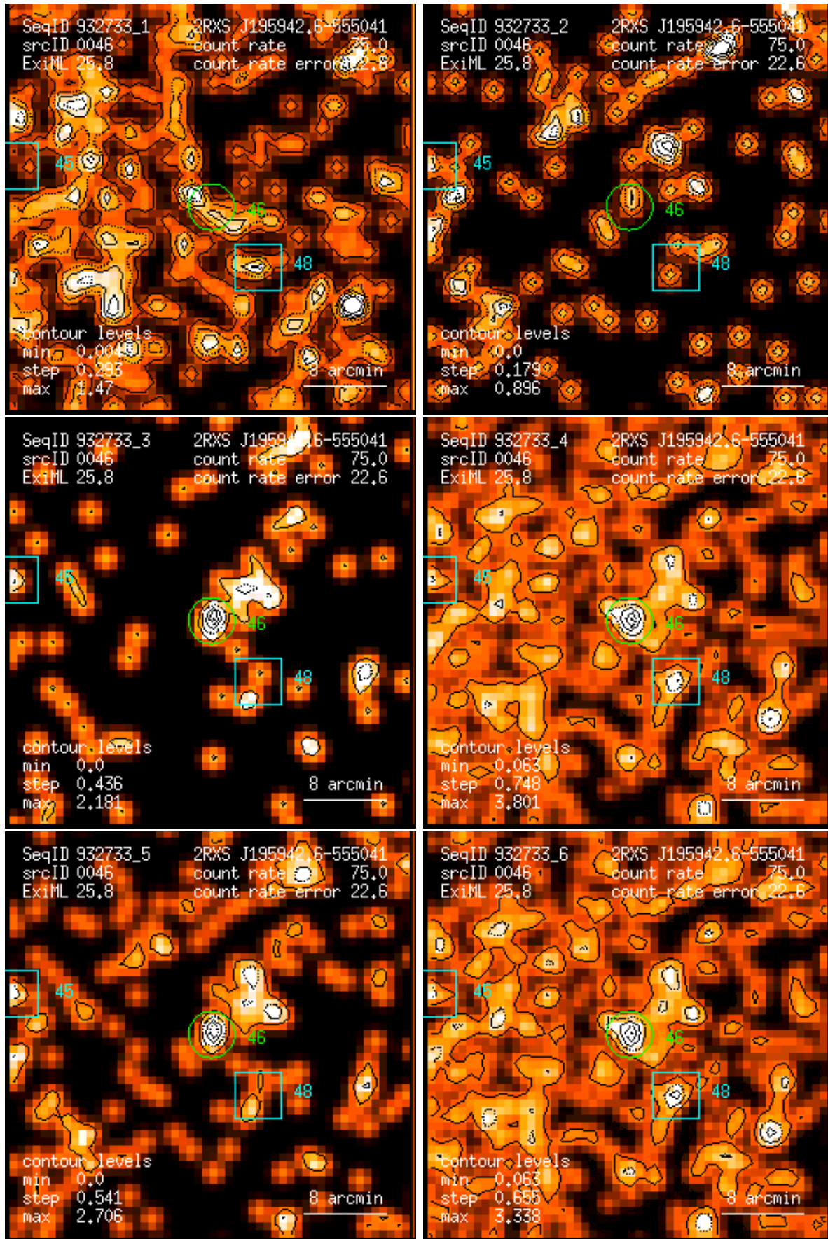
Figure 46: RASS 932733: detection 0046: band rate images, Gaussian filter: (1) PSPC channels 11 – 41, (2) 52 – 90, (3) 91 – 201, (4) 11 – 235, (5) 52 – 201, (6) 11 – 201. Broad band rates in counts/ks. Band rate contour levels in counts/ks/arcmin 2 .
