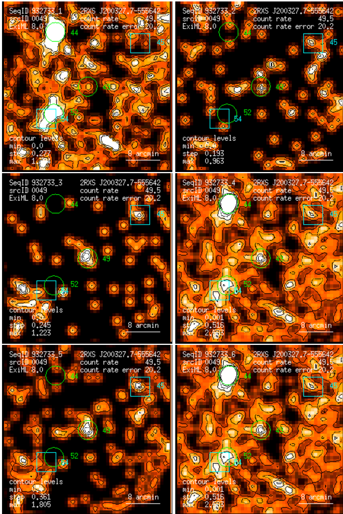
Figure 49: RASS 932733: detection 0049: band rate images, Gaussian filter: (1) PSPC channels 11 – 41, (2) 52 – 90, (3) 91 – 201, (4) 11 – 235, (5) 52 – 201, (6) 11 – 201. Broad band rates in counts/ks. Band rate contour levels in counts/ks/arcmin 2 .
