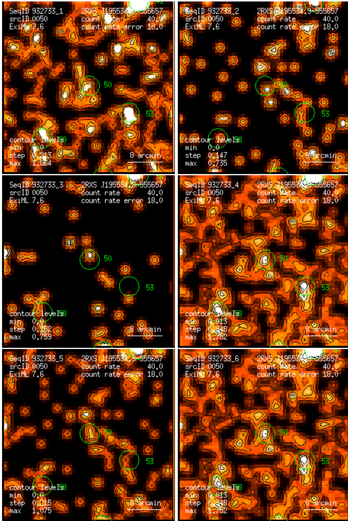
Figure 50: RASS 932733: detection 0050: band rate images, Gaussian filter: (1) PSPC channels 11 – 41, (2) 52 – 90, (3) 91 – 201, (4) 11 – 235, (5) 52 – 201, (6) 11 – 201. Broad band rates in counts/ks. Band rate contour levels in counts/ks/arcmin 2 .
