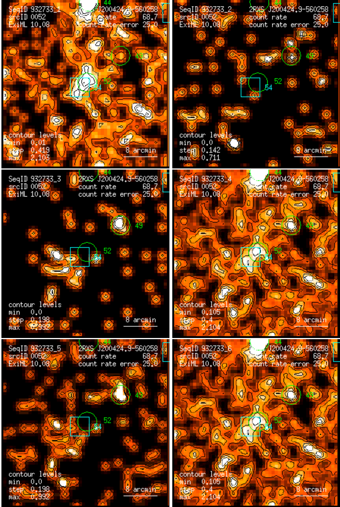
Figure 52: RASS 932733: detection 0052: band rate images, Gaussian filter: (1) PSPC channels 11 – 41, (2) 52 – 90, (3) 91 – 201, (4) 11 – 235, (5) 52 – 201, (6) 11 – 201. Broad band rates in counts/ks. Band rate contour levels in counts/ks/arcmin 2 .
