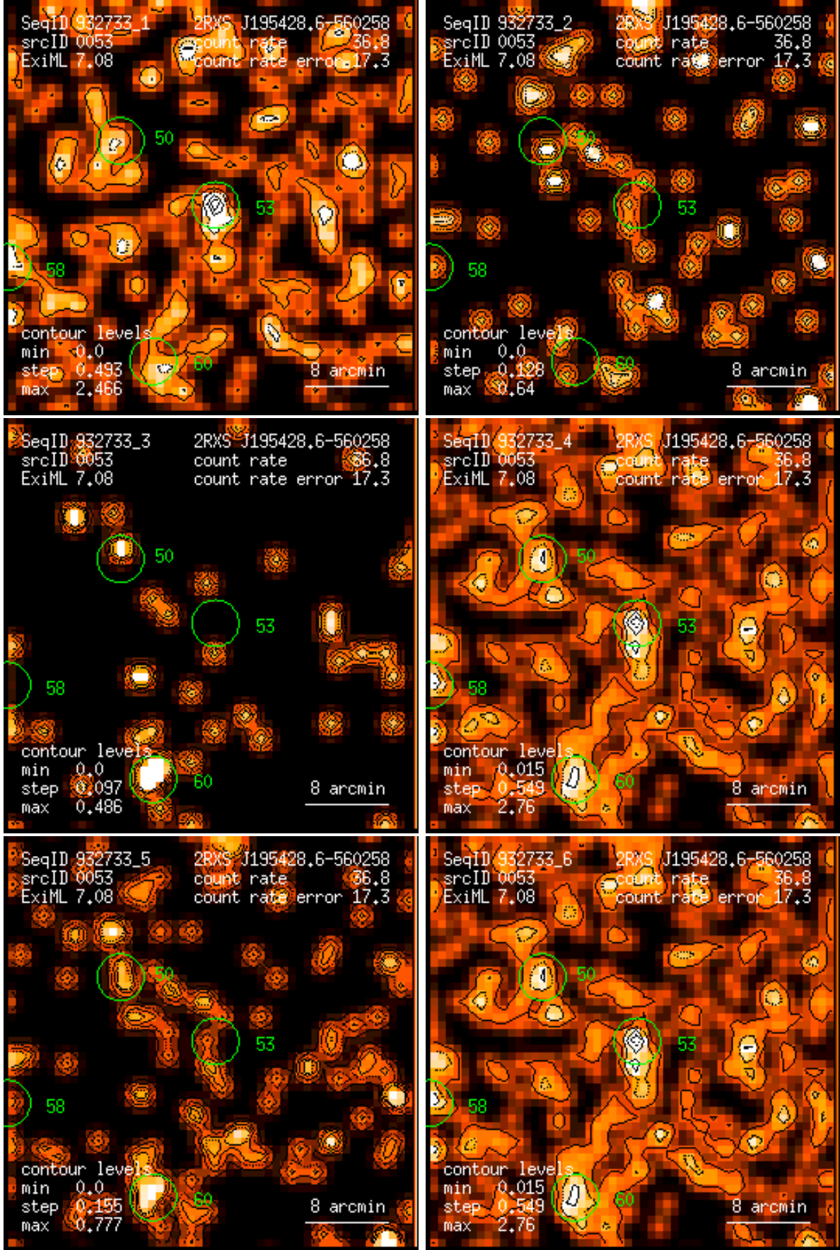
Figure 53: RASS 932733: detection 0053: band rate images, Gaussian filter: (1) PSPC channels 11 – 41, (2) 52 – 90, (3) 91 – 201, (4) 11 – 235, (5) 52 – 201, (6) 11 – 201. Broad band rates in counts/ks. Band rate contour levels in counts/ks/arcmin 2 .
