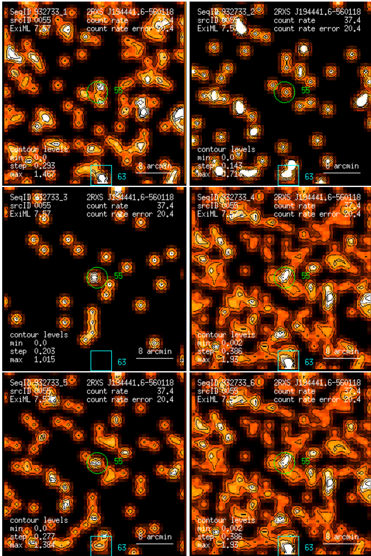
Figure 55: RASS 932733: detection 0055: band rate images, Gaussian filter: (1) PSPC channels 11 – 41, (2) 52 – 90, (3) 91 – 201, (4) 11 – 235, (5) 52 – 201, (6) 11 – 201. Broad band rates in counts/ks. Band rate contour levels in counts/ks/arcmin 2 .
