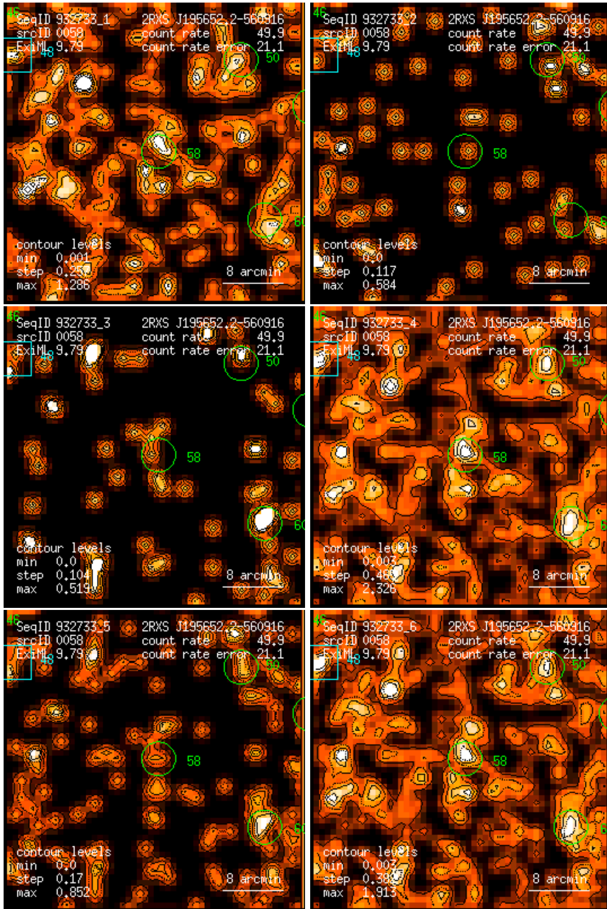
Figure 58: RASS 932733: detection 0058: band rate images, Gaussian filter: (1) PSPC channels 11 – 41, (2) 52 – 90, (3) 91 – 201, (4) 11 – 235, (5) 52 – 201, (6) 11 – 201. Broad band rates in counts/ks. Band rate contour levels in counts/ks/arcmin 2 .
