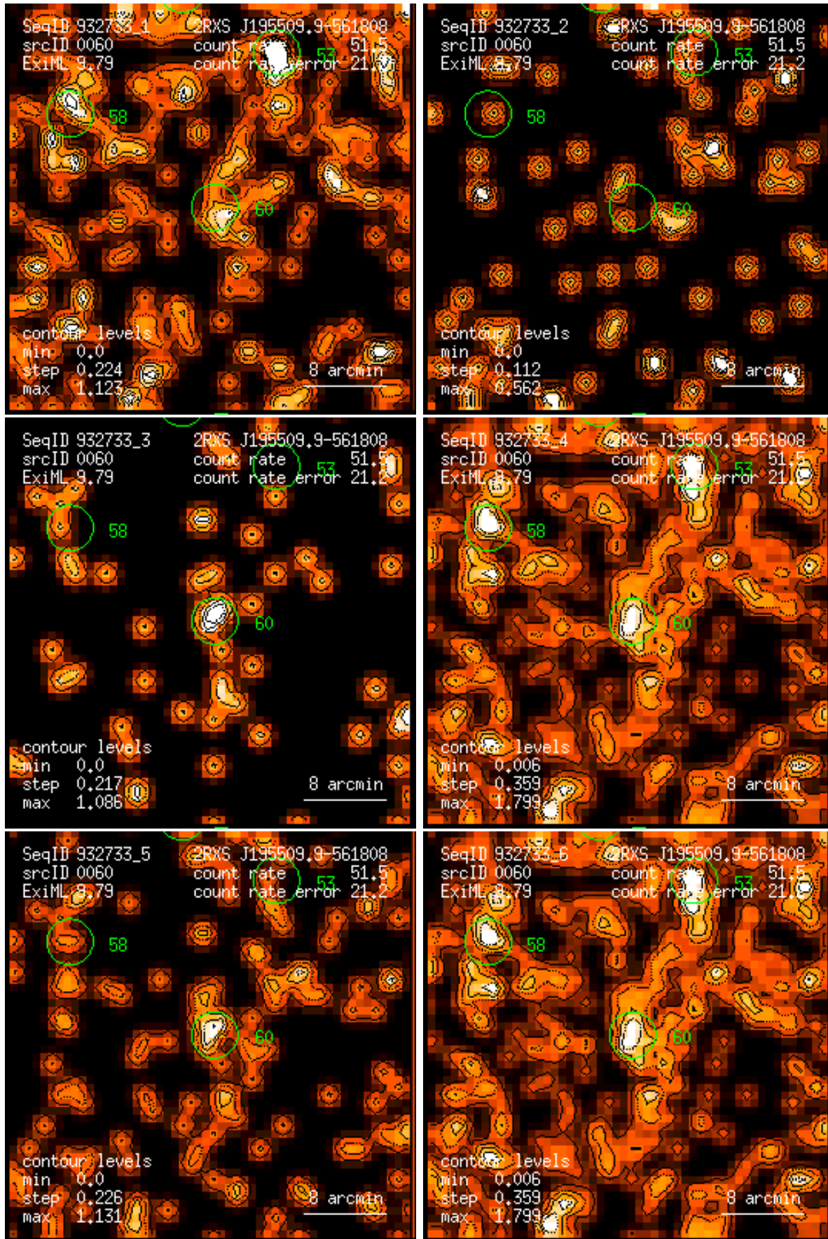
Figure 60: RASS 932733: detection 0060: band rate images, Gaussian filter: (1) PSPC channels 11 – 41, (2) 52 – 90, (3) 91 – 201, (4) 11 – 235, (5) 52 – 201, (6) 11 – 201. Broad band rates in counts/ks. Band rate contour levels in counts/ks/arcmin 2 .
