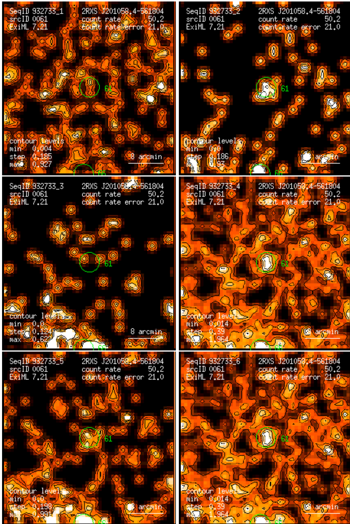
Figure 61: RASS 932733: detection 0061: band rate images, Gaussian filter: (1) PSPC channels 11 – 41, (2) 52 – 90, (3) 91 – 201, (4) 11 – 235, (5) 52 – 201, (6) 11 – 201. Broad band rates in counts/ks. Band rate contour levels in counts/ks/arcmin 2 .
