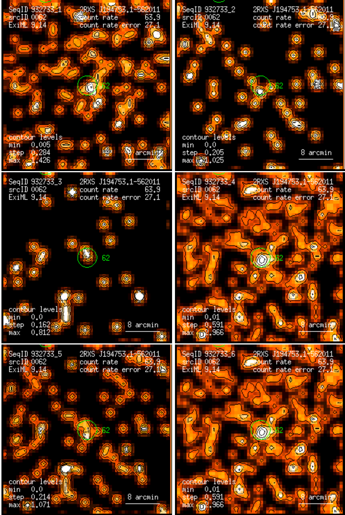
Figure 62: RASS 932733: detection 0062: band rate images, Gaussian filter: (1) PSPC channels 11 – 41, (2) 52 – 90, (3) 91 – 201, (4) 11 – 235, (5) 52 – 201, (6) 11 – 201. Broad band rates in counts/ks. Band rate contour levels in counts/ks/arcmin 2 .
