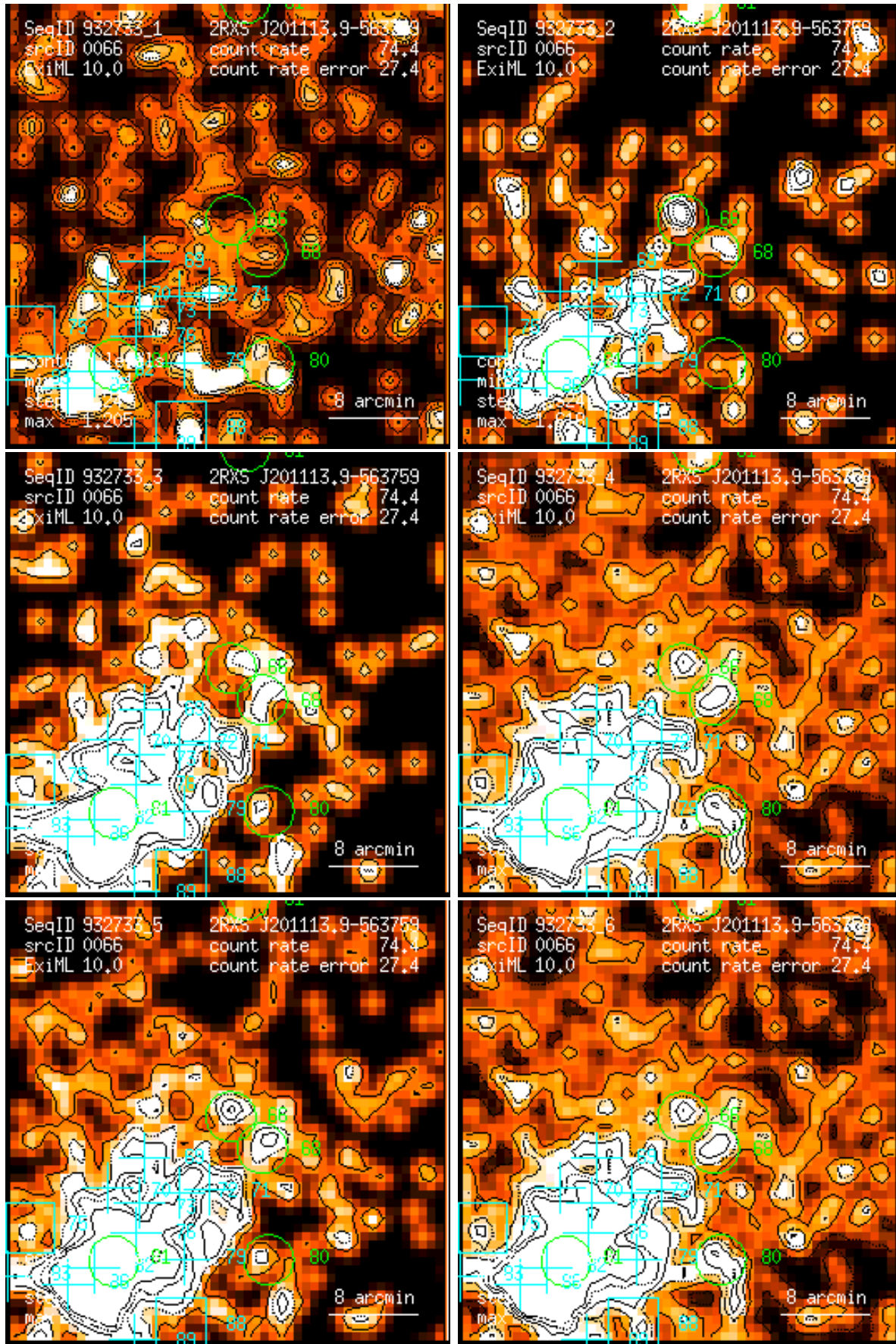
Figure 66: RASS 932733: detection 0066: band rate images, Gaussian filter: (1) PSPC channels 11 – 41, (2) 52 – 90, (3) 91 – 201, (4) 11 – 235, (5) 52 – 201, (6) 11 – 201. Broad band rates in counts/ks. Band rate contour levels in counts/ks/arcmin 2 .
