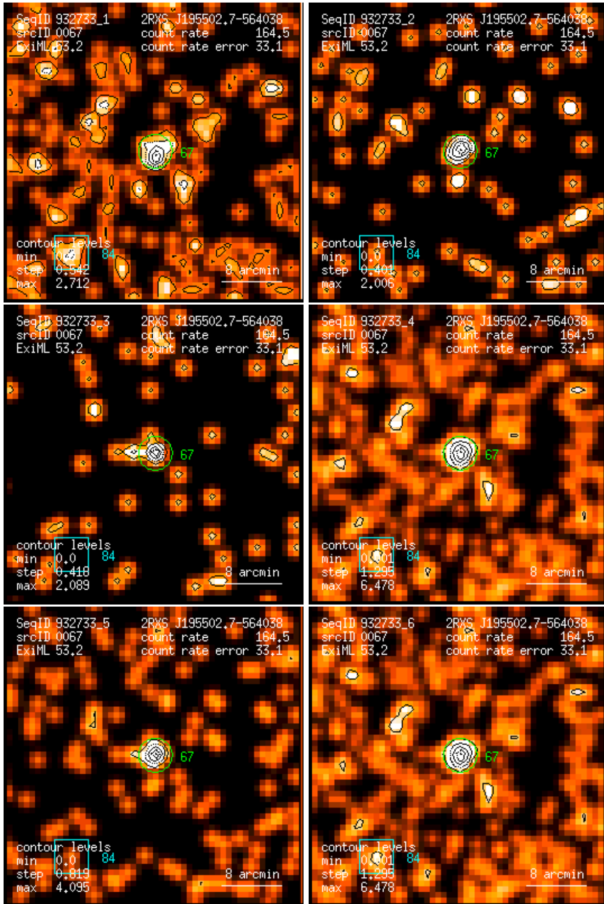
Figure 67: RASS 932733: detection 0067: band rate images, Gaussian filter: (1) PSPC channels 11 – 41, (2) 52 – 90, (3) 91 – 201, (4) 11 – 235, (5) 52 – 201, (6) 11 – 201. Broad band rates in counts/ks. Band rate contour levels in counts/ks/arcmin 2 .
