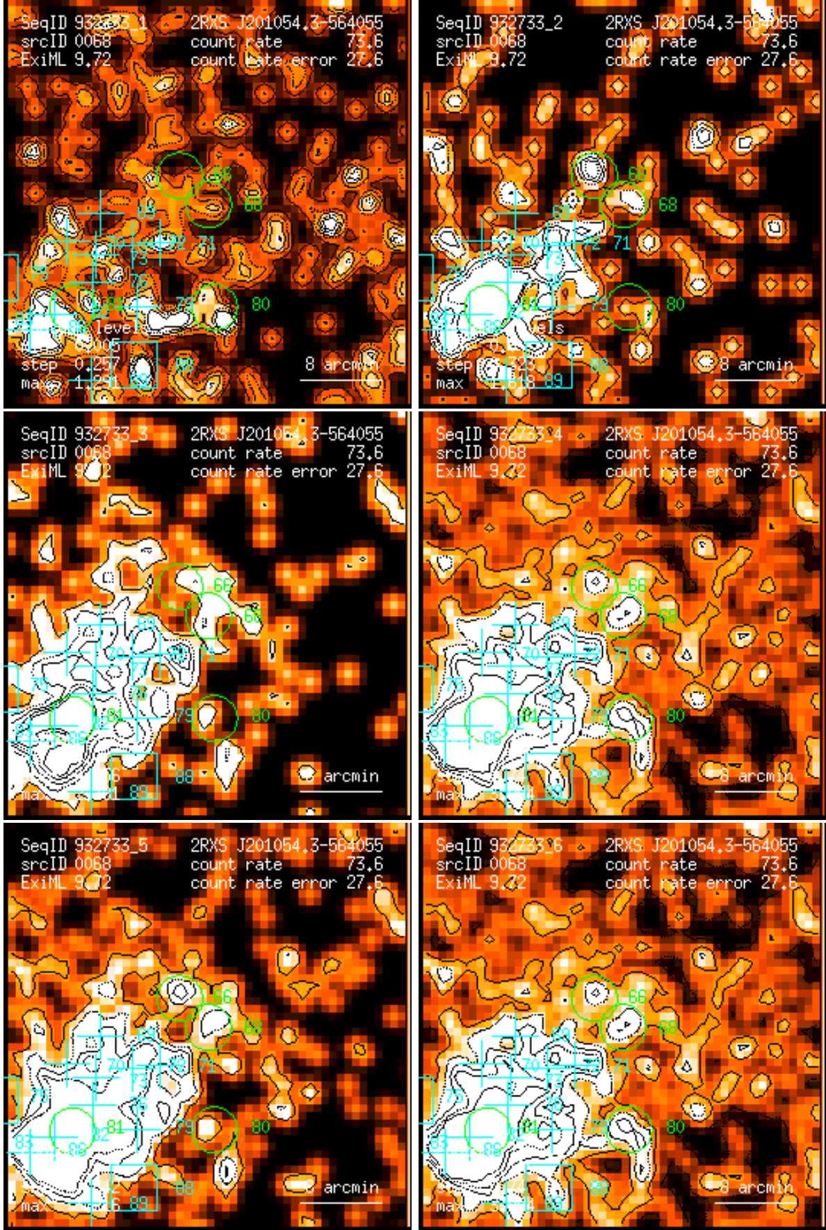
Figure 68: RASS 932733: detection 0068: band rate images, Gaussian filter: (1) PSPC channels 11 – 41, (2) 52 – 90, (3) 91 – 201, (4) 11 – 235, (5) 52 – 201, (6) 11 – 201. Broad band rates in counts/ks. Band rate contour levels in counts/ks/arcmin 2 .
