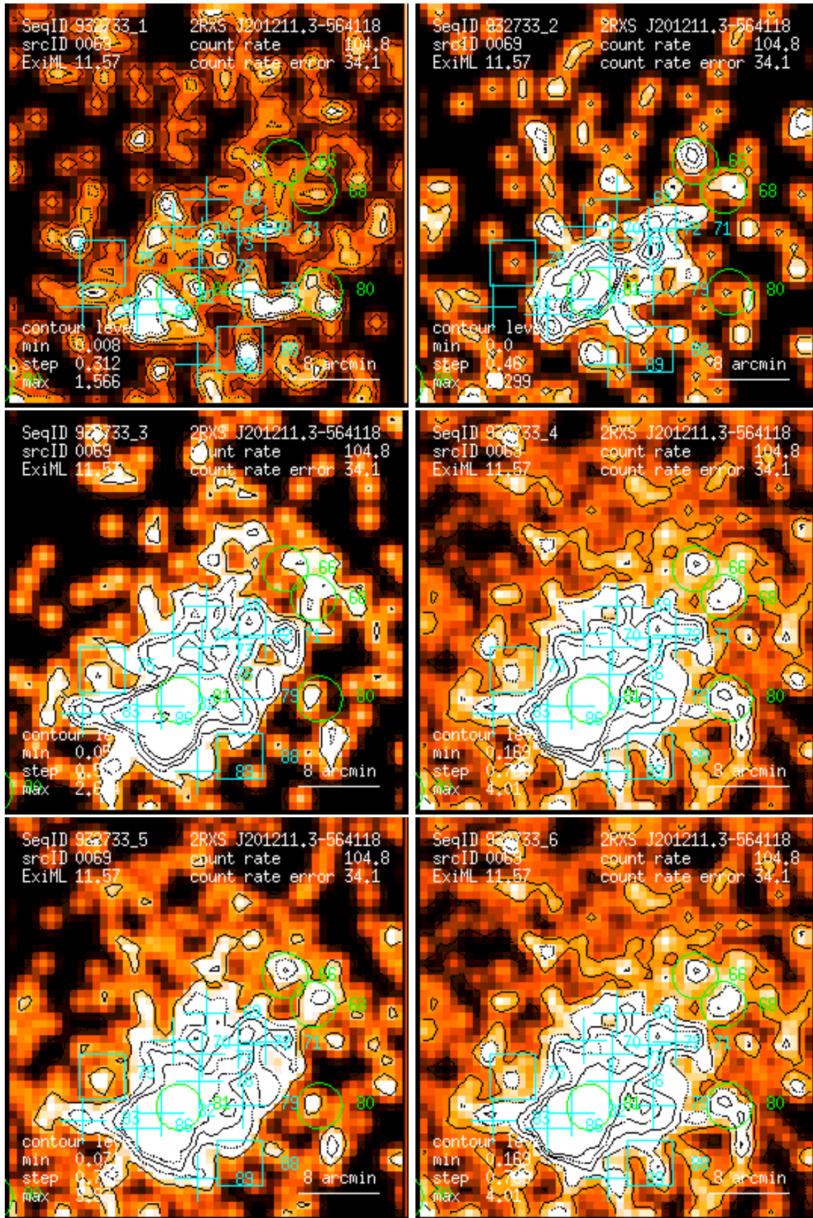
Figure 69: RASS 932733: detection 0069: band rate images, Gaussian filter: (1) PSPC channels 11 – 41, (2) 52 – 90, (3) 91 – 201, (4) 11 – 235, (5) 52 – 201, (6) 11 – 201. Broad band rates in counts/ks. Band rate contour levels in counts/ks/arcmin 2 .
