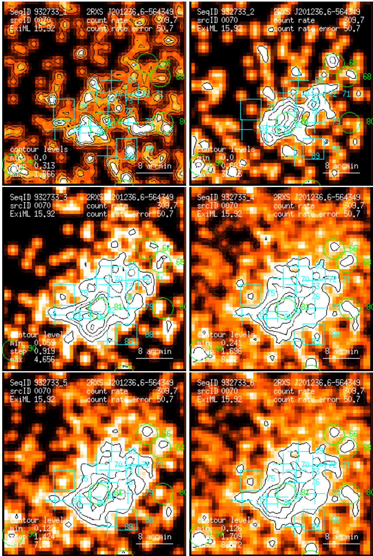
Figure 70: RASS 932733: detection 0070: band rate images, Gaussian filter: (1) PSPC channels 11 – 41, (2) 52 – 90, (3) 91 – 201, (4) 11 – 235, (5) 52 – 201, (6) 11 – 201. Broad band rates in counts/ks. Band rate contour levels in counts/ks/arcmin 2 .
