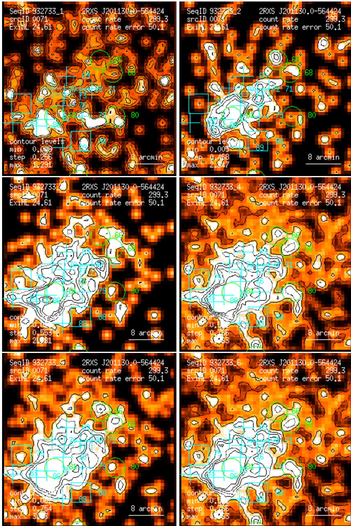
Figure 71: RASS 932733: detection 0071: band rate images, Gaussian filter: (1) PSPC channels 11 – 41, (2) 52 – 90, (3) 91 – 201, (4) 11 – 235, (5) 52 – 201, (6) 11 – 201. Broad band rates in counts/ks. Band rate contour levels in counts/ks/arcmin 2 .
