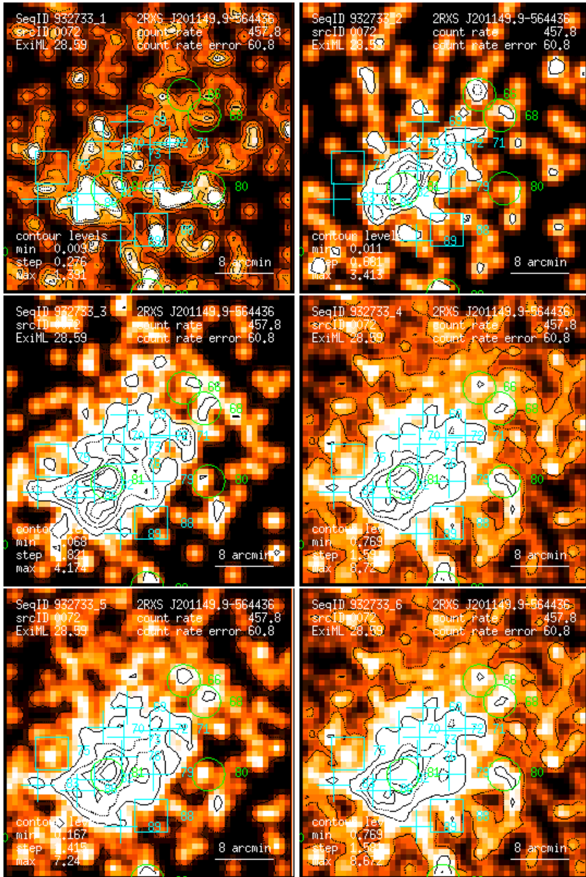
Figure 72: RASS 932733: detection 0072: band rate images, Gaussian filter: (1) PSPC channels 11 – 41, (2) 52 – 90, (3) 91 – 201, (4) 11 – 235, (5) 52 – 201, (6) 11 – 201. Broad band rates in counts/ks. Band rate contour levels in counts/ks/arcmin 2 .
