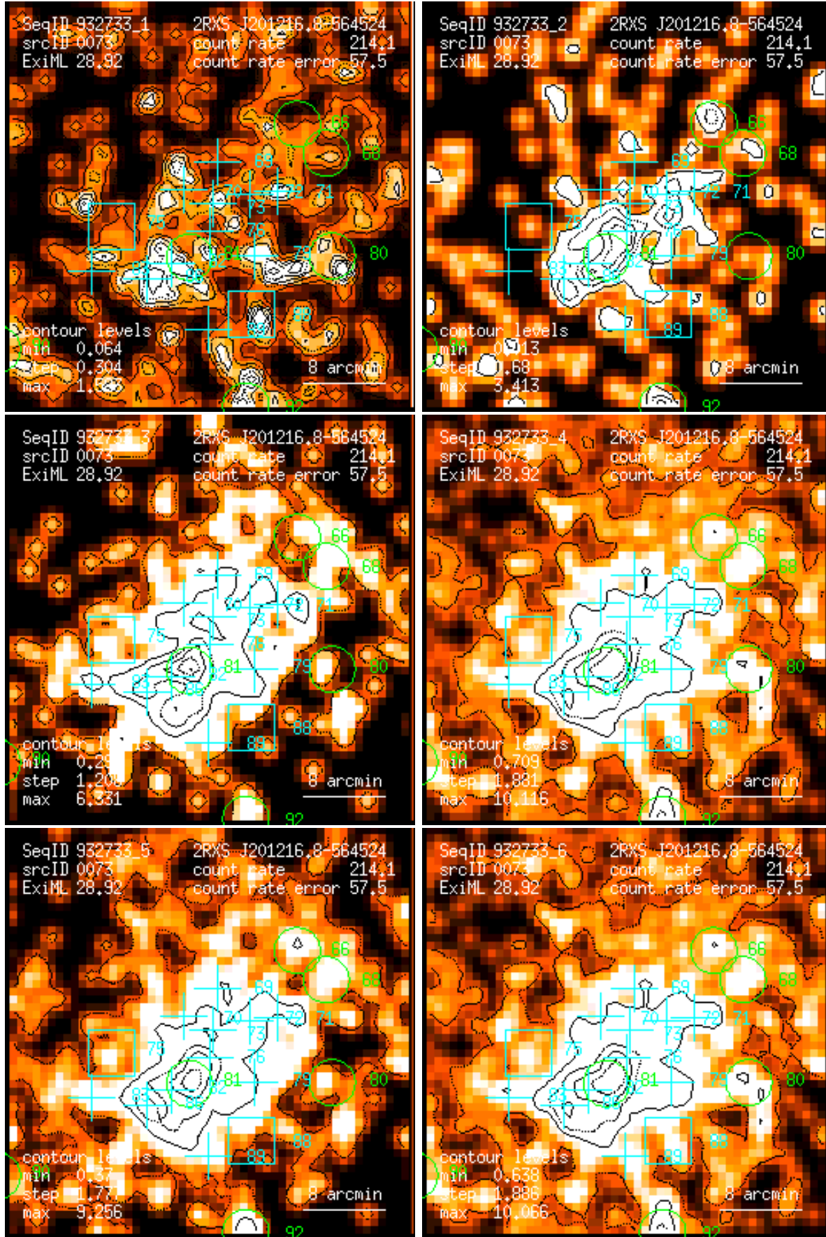
Figure 73: RASS 932733: detection 0073: band rate images, Gaussian filter: (1) PSPC channels 11 – 41, (2) 52 – 90, (3) 91 – 201, (4) 11 – 235, (5) 52 – 201, (6) 11 – 201. Broad band rates in counts/ks. Band rate contour levels in counts/ks/arcmin 2 .
