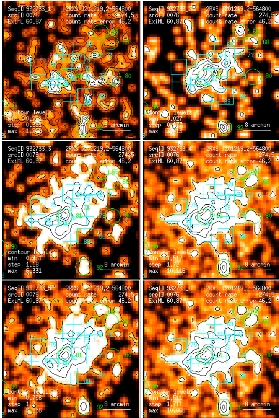
Figure 76: RASS 932733: detection 0076: band rate images, Gaussian filter: (1) PSPC channels 11 – 41, (2) 52 – 90, (3) 91 – 201, (4) 11 – 235, (5) 52 – 201, (6) 11 – 201. Broad band rates in counts/ks. Band rate contour levels in counts/ks/arcmin 2 .
