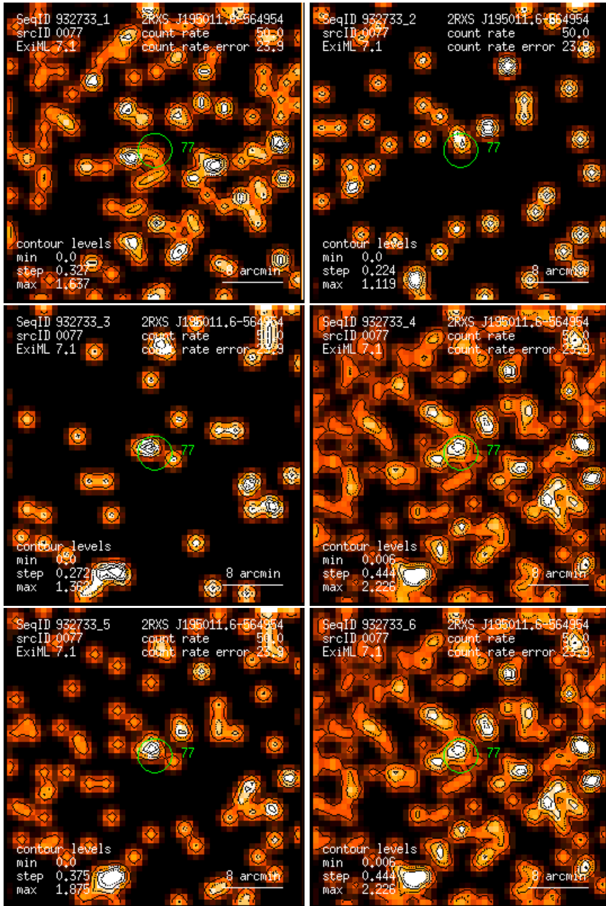
Figure 77: RASS 932733: detection 0077: band rate images, Gaussian filter: (1) PSPC channels 11 – 41, (2) 52 – 90, (3) 91 – 201, (4) 11 – 235, (5) 52 – 201, (6) 11 – 201. Broad band rates in counts/ks. Band rate contour levels in counts/ks/arcmin 2 .
