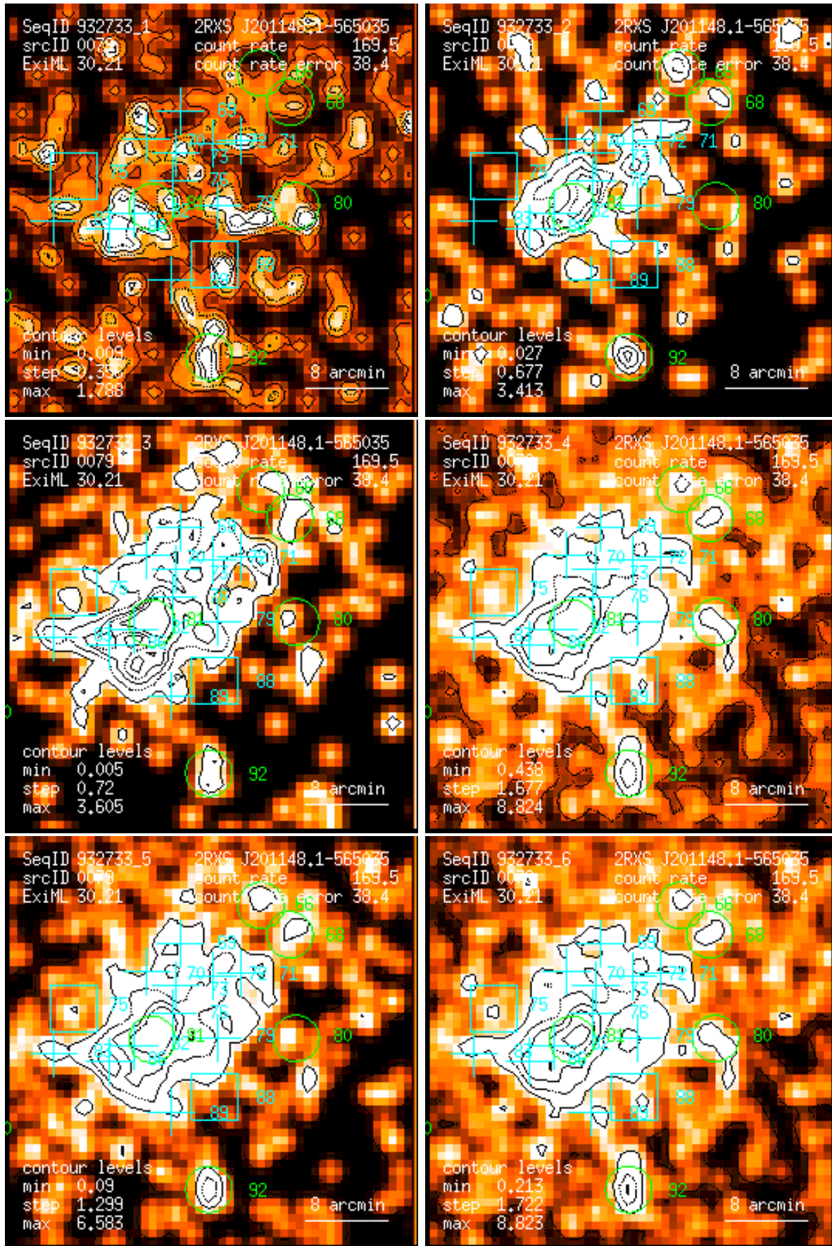
Figure 79: RASS 932733: detection 0079: band rate images, Gaussian filter: (1) PSPC channels 11 – 41, (2) 52 – 90, (3) 91 – 201, (4) 11 – 235, (5) 52 – 201, (6) 11 – 201. Broad band rates in counts/ks. Band rate contour levels in counts/ks/arcmin 2 .
