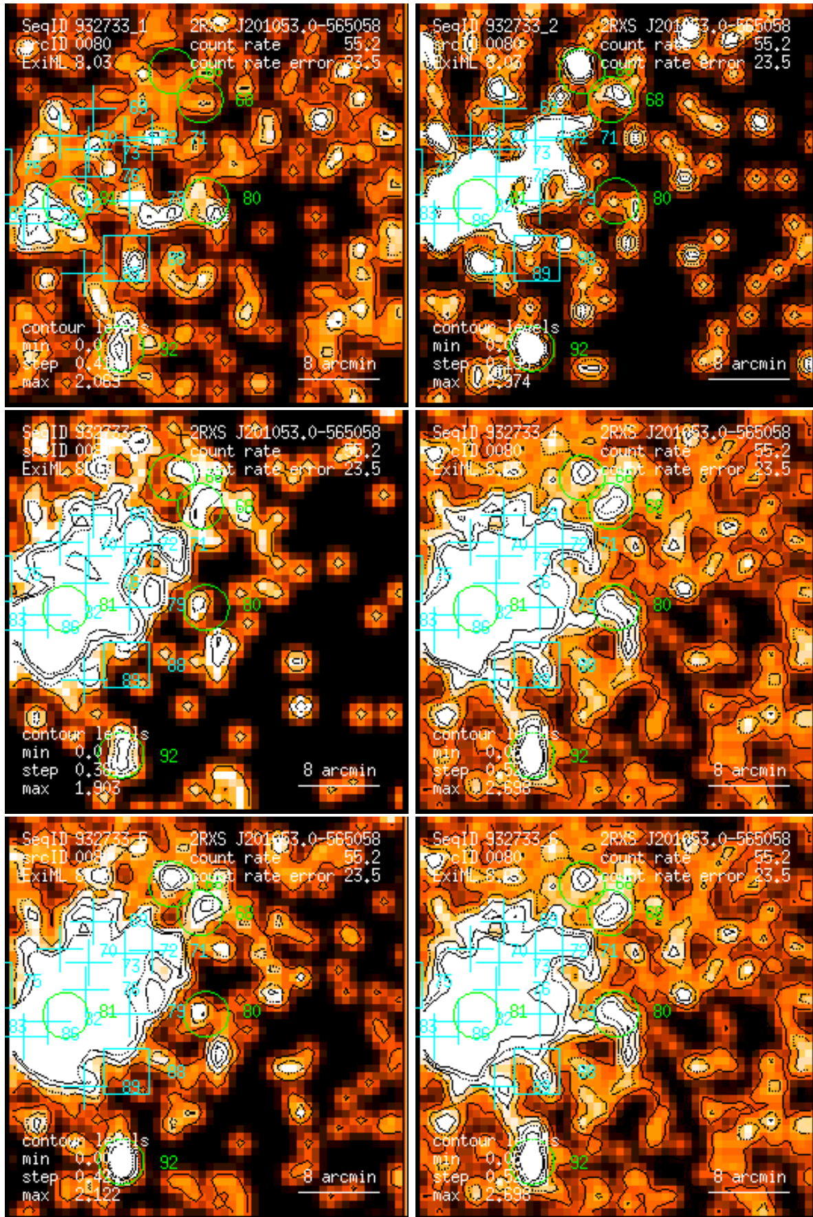
Figure 80: RASS 932733: detection 0080: band rate images, Gaussian filter: (1) PSPC channels 11 – 41, (2) 52 – 90, (3) 91 – 201, (4) 11 – 235, (5) 52 – 201, (6) 11 – 201. Broad band rates in counts/ks. Band rate contour levels in counts/ks/arcmin 2 .
