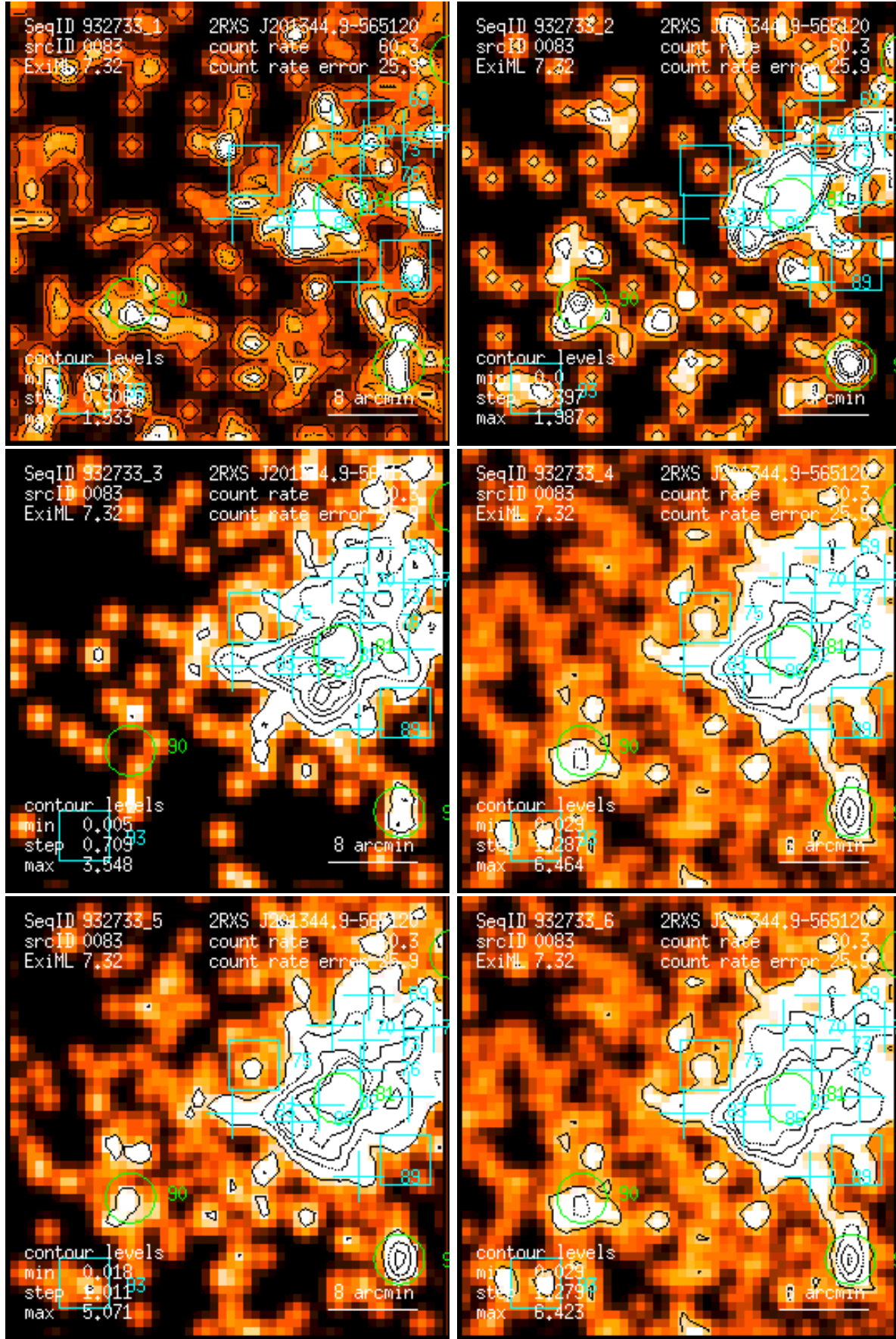
Figure 83: RASS 932733: detection 0083: band rate images, Gaussian filter: (1) PSPC channels 11 – 41, (2) 52 – 90, (3) 91 – 201, (4) 11 – 235, (5) 52 – 201, (6) 11 – 201. Broad band rates in counts/ks. Band rate contour levels in counts/ks/arcmin 2 .
