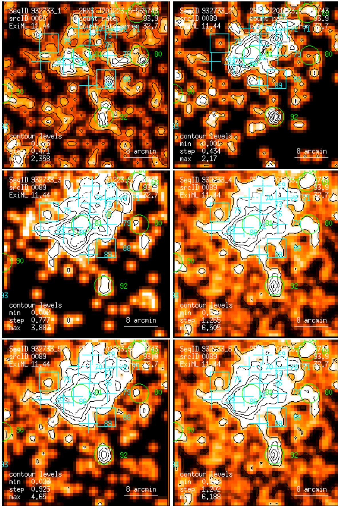
Figure 89: RASS 932733: detection 0089: band rate images, Gaussian filter: (1) PSPC channels 11 – 41, (2) 52 – 90, (3) 91 – 201, (4) 11 – 235, (5) 52 – 201, (6) 11 – 201. Broad band rates in counts/ks. Band rate contour levels in counts/ks/arcmin 2 .
