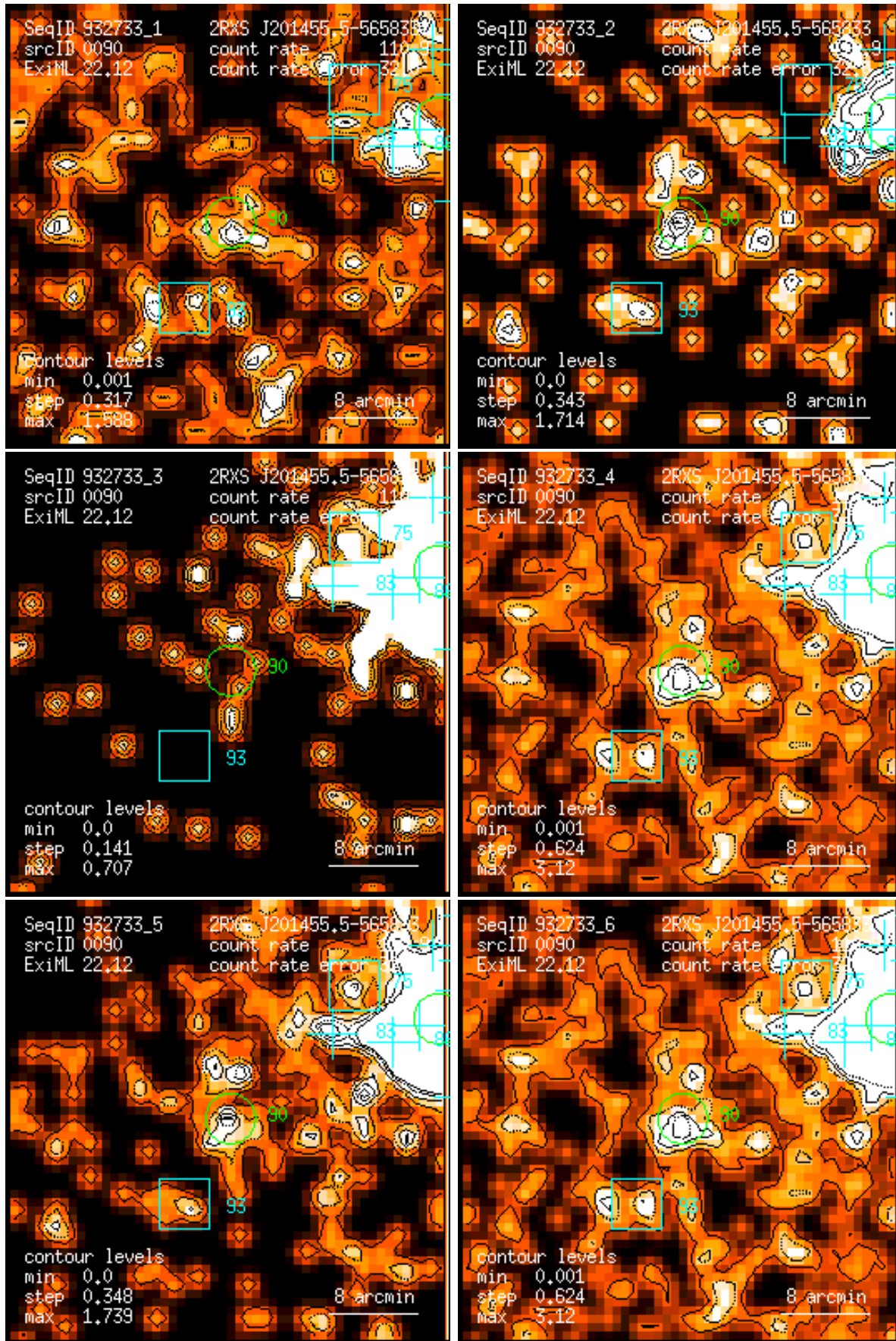
Figure 90: RASS 932733: detection 0090: band rate images, Gaussian filter: (1) PSPC channels 11 – 41, (2) 52 – 90, (3) 91 – 201, (4) 11 – 235, (5) 52 – 201, (6) 11 – 201. Broad band rates in counts/ks. Band rate contour levels in counts/ks/arcmin 2 .
