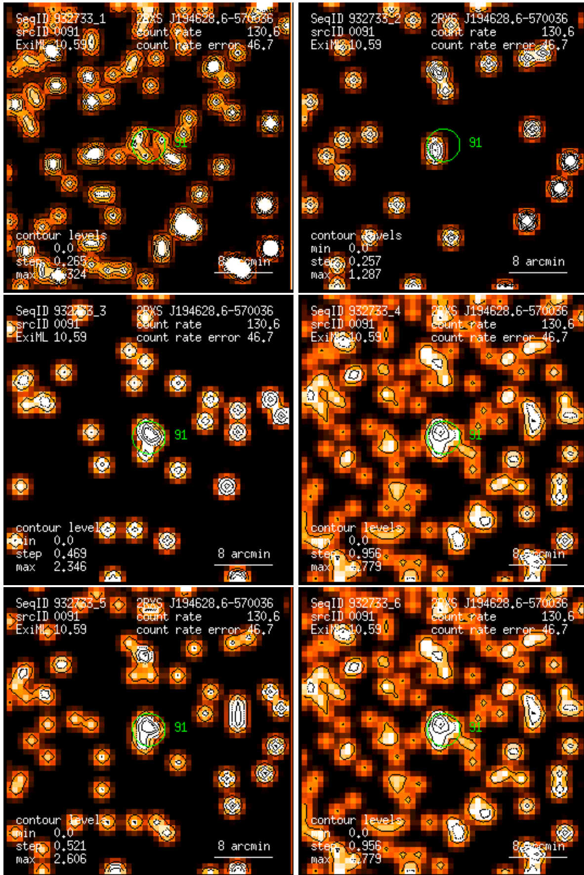
Figure 91: RASS 932733: detection 0091: band rate images, Gaussian filter: (1) PSPC channels 11 – 41, (2) 52 – 90, (3) 91 – 201, (4) 11 – 235, (5) 52 – 201, (6) 11 – 201. Broad band rates in counts/ks. Band rate contour levels in counts/ks/arcmin 2 .
