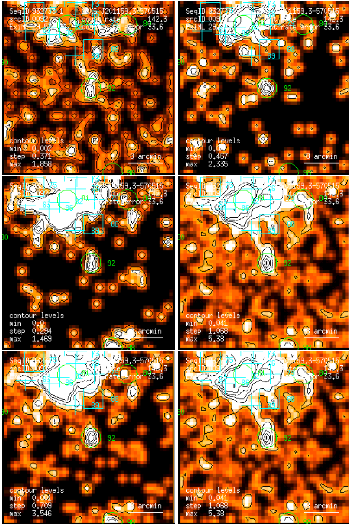
Figure 92: RASS 932733: detection 0092: band rate images, Gaussian filter: (1) PSPC channels 11 – 41, (2) 52 – 90, (3) 91 – 201, (4) 11 – 235, (5) 52 – 201, (6) 11 – 201. Broad band rates in counts/ks. Band rate contour levels in counts/ks/arcmin 2 .
