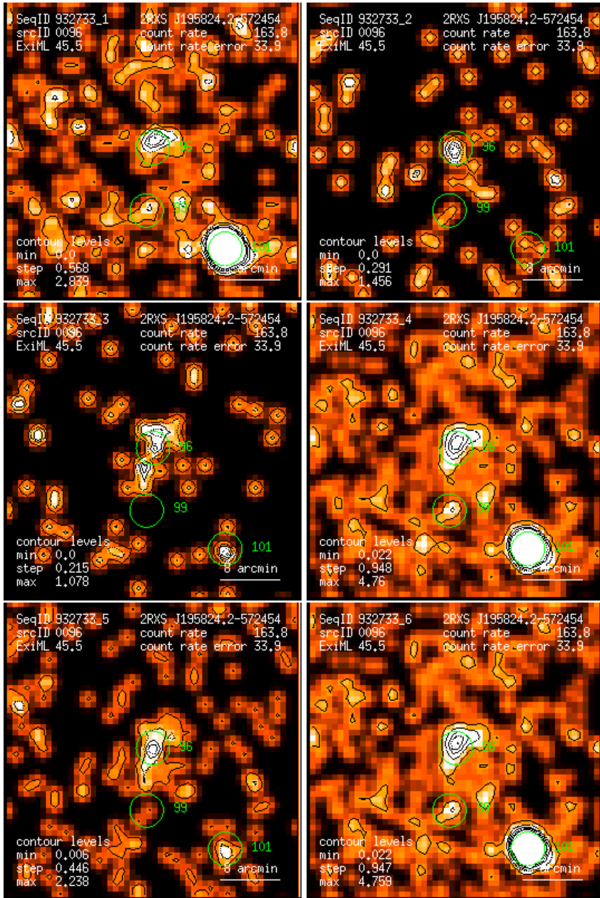
Figure 96: RASS 932733: detection 0096: band rate images, Gaussian filter: (1) PSPC channels 11 – 41, (2) 52 – 90, (3) 91 – 201, (4) 11 – 235, (5) 52 – 201, (6) 11 – 201. Broad band rates in counts/ks. Band rate contour levels in counts/ks/arcmin 2 .
