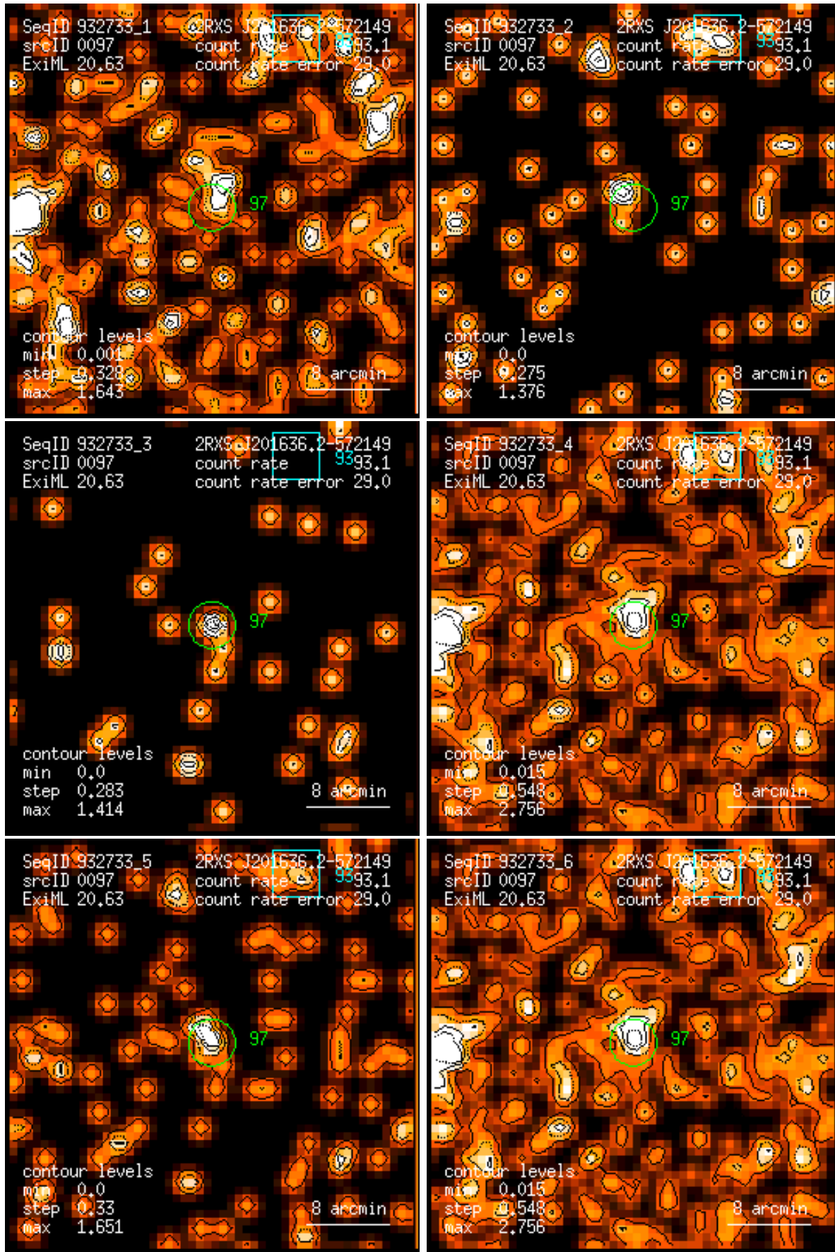
Figure 97: RASS 932733: detection 0097: band rate images, Gaussian filter: (1) PSPC channels 11 – 41, (2) 52 – 90, (3) 91 – 201, (4) 11 – 235, (5) 52 – 201, (6) 11 – 201. Broad band rates in counts/ks. Band rate contour levels in counts/ks/arcmin 2 .
