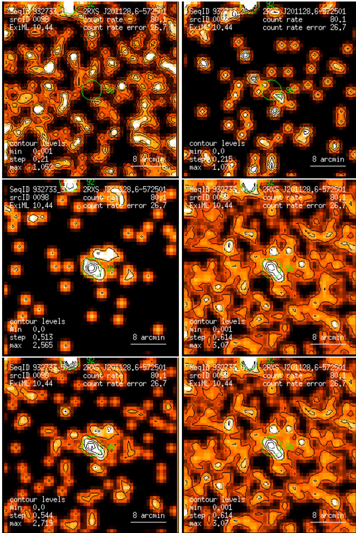
Figure 98: RASS 932733: detection 0098: band rate images, Gaussian filter: (1) PSPC channels 11 – 41, (2) 52 – 90, (3) 91 – 201, (4) 11 – 235, (5) 52 – 201, (6) 11 – 201. Broad band rates in counts/ks. Band rate contour levels in counts/ks/arcmin 2 .
