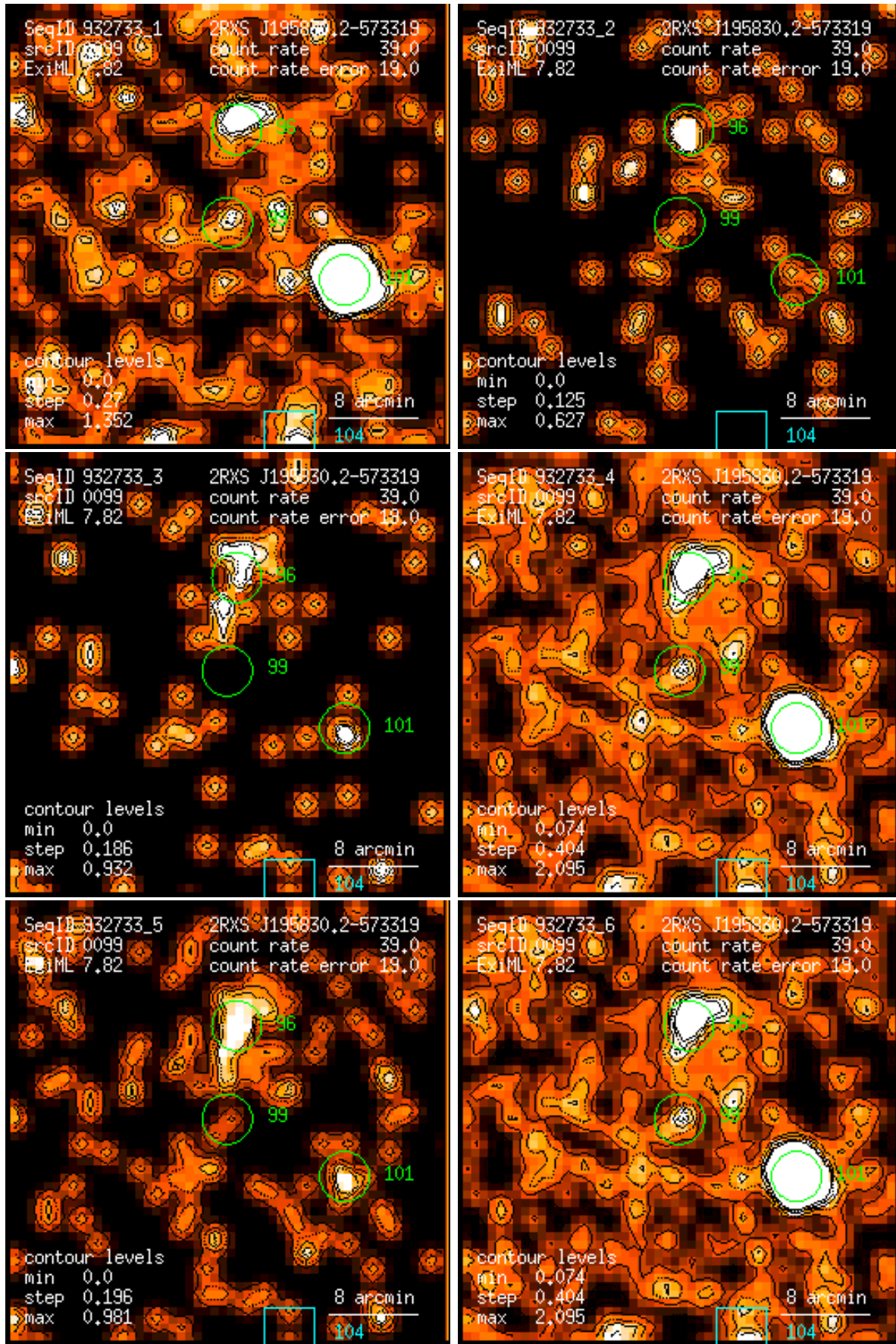
Figure 99: RASS 932733: detection 0099: band rate images, Gaussian filter: (1) PSPC channels 11 – 41, (2) 52 – 90, (3) 91 – 201, (4) 11 – 235, (5) 52 – 201, (6) 11 – 201. Broad band rates in counts/ks. Band rate contour levels in counts/ks/arcmin 2 .
