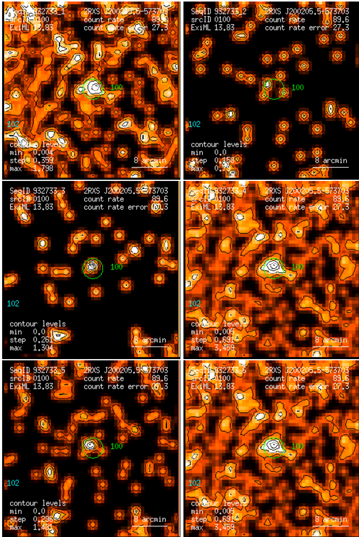
Figure 100: RASS 932733: detection 0100: band rate images, Gaussian filter: (1) PSPC channels 11 – 41, (2) 52 – 90, (3) 91 – 201, (4) 11 – 235, (5) 52 – 201, (6) 11 – 201. Broad band rates in counts/ks. Band rate contour levels in counts/ks/arcmin 2 .
