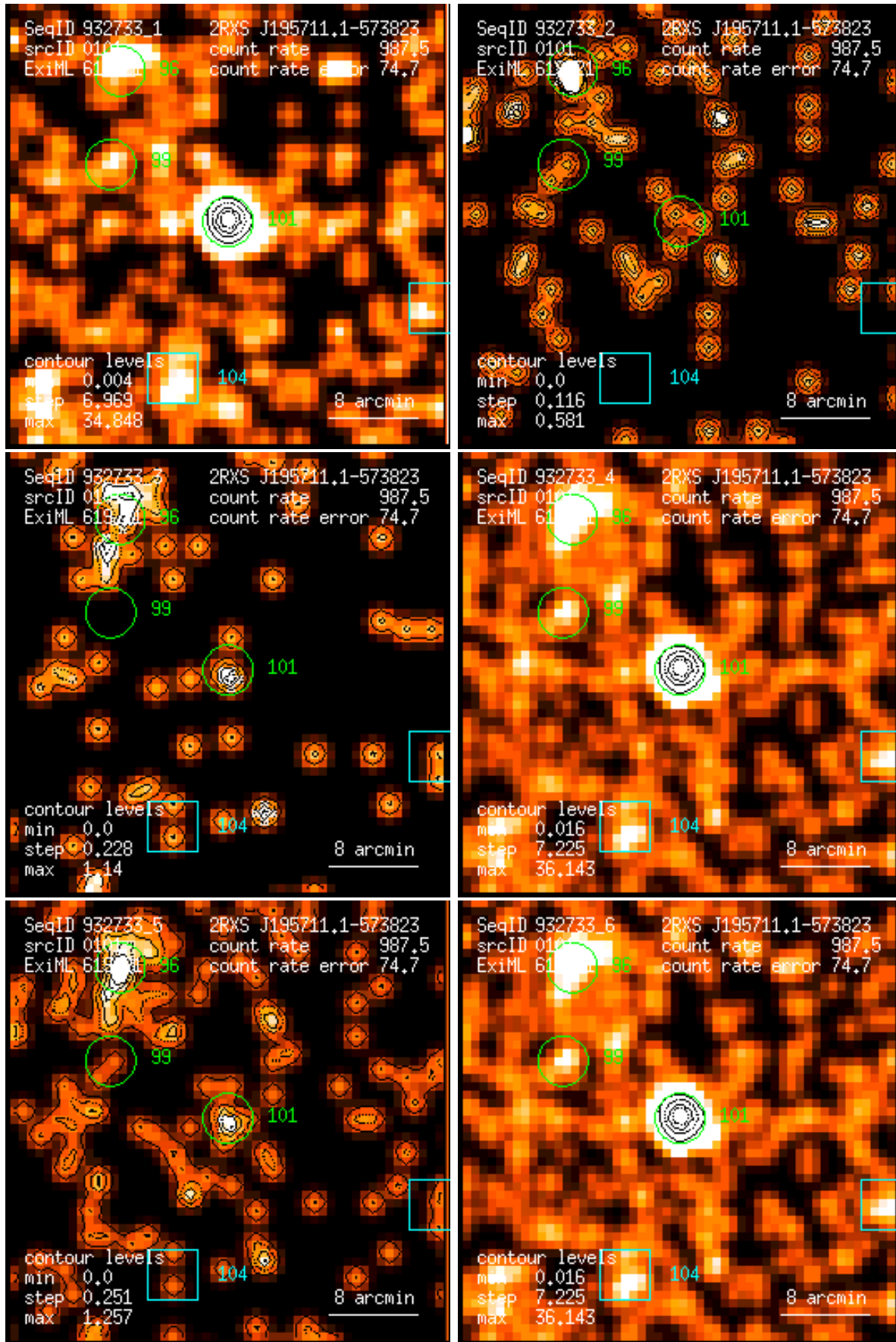
Figure 101: RASS 932733: detection 0101: band rate images, Gaussian filter: (1) PSPC channels 11 – 41, (2) 52 – 90, (3) 91 – 201, (4) 11 – 235, (5) 52 – 201, (6) 11 – 201. Broad band rates in counts/ks. Band rate contour levels in counts/ks/arcmin 2 .
