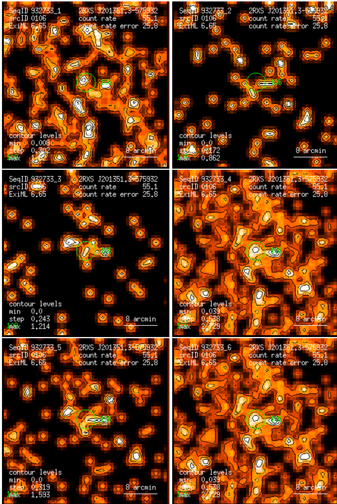
Figure 106: RASS 932733: detection 0106: band rate images, Gaussian filter: (1) PSPC channels 11 – 41, (2) 52 – 90, (3) 91 – 201, (4) 11 – 235, (5) 52 – 201, (6) 11 – 201. Broad band rates in counts/ks. Band rate contour levels in counts/ks/arcmin 2 .
