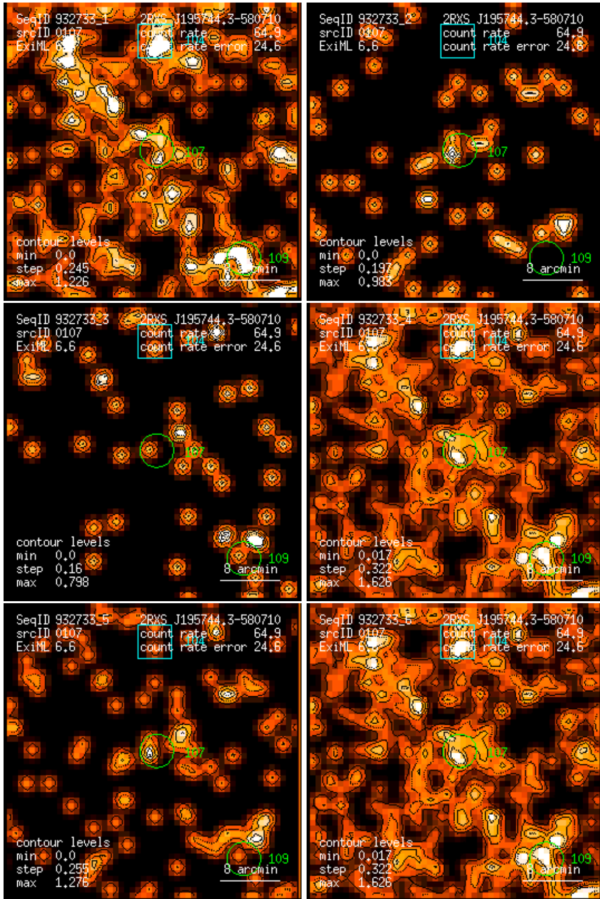
Figure 107: RASS 932733: detection 0107: band rate images, Gaussian filter: (1) PSPC channels 11 – 41, (2) 52 – 90, (3) 91 – 201, (4) 11 – 235, (5) 52 – 201, (6) 11 – 201. Broad band rates in counts/ks. Band rate contour levels in counts/ks/arcmin 2 .
