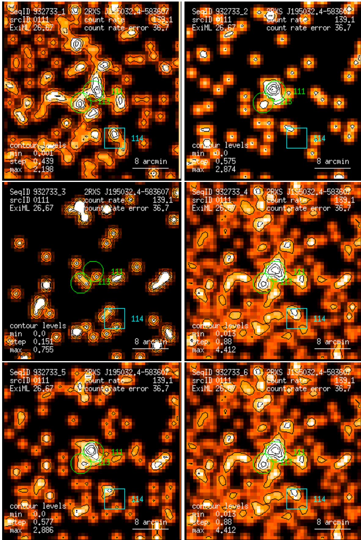
Figure 111: RASS 932733: detection 0111: band rate images, Gaussian filter: (1) PSPC channels 11 – 41, (2) 52 – 90, (3) 91 – 201, (4) 11 – 235, (5) 52 – 201, (6) 11 – 201. Broad band rates in counts/ks. Band rate contour levels in counts/ks/arcmin 2 .
