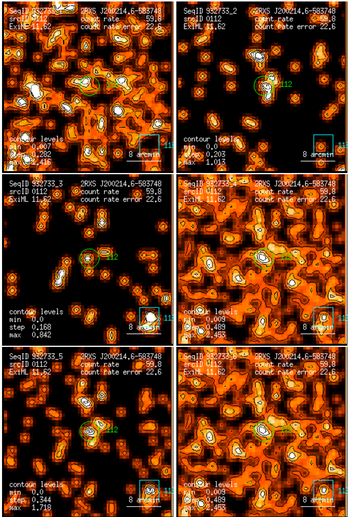
Figure 112: RASS 932733: detection 0112: band rate images, Gaussian filter: (1) PSPC channels 11 – 41, (2) 52 – 90, (3) 91 – 201, (4) 11 – 235, (5) 52 – 201, (6) 11 – 201. Broad band rates in counts/ks. Band rate contour levels in counts/ks/arcmin 2 .
