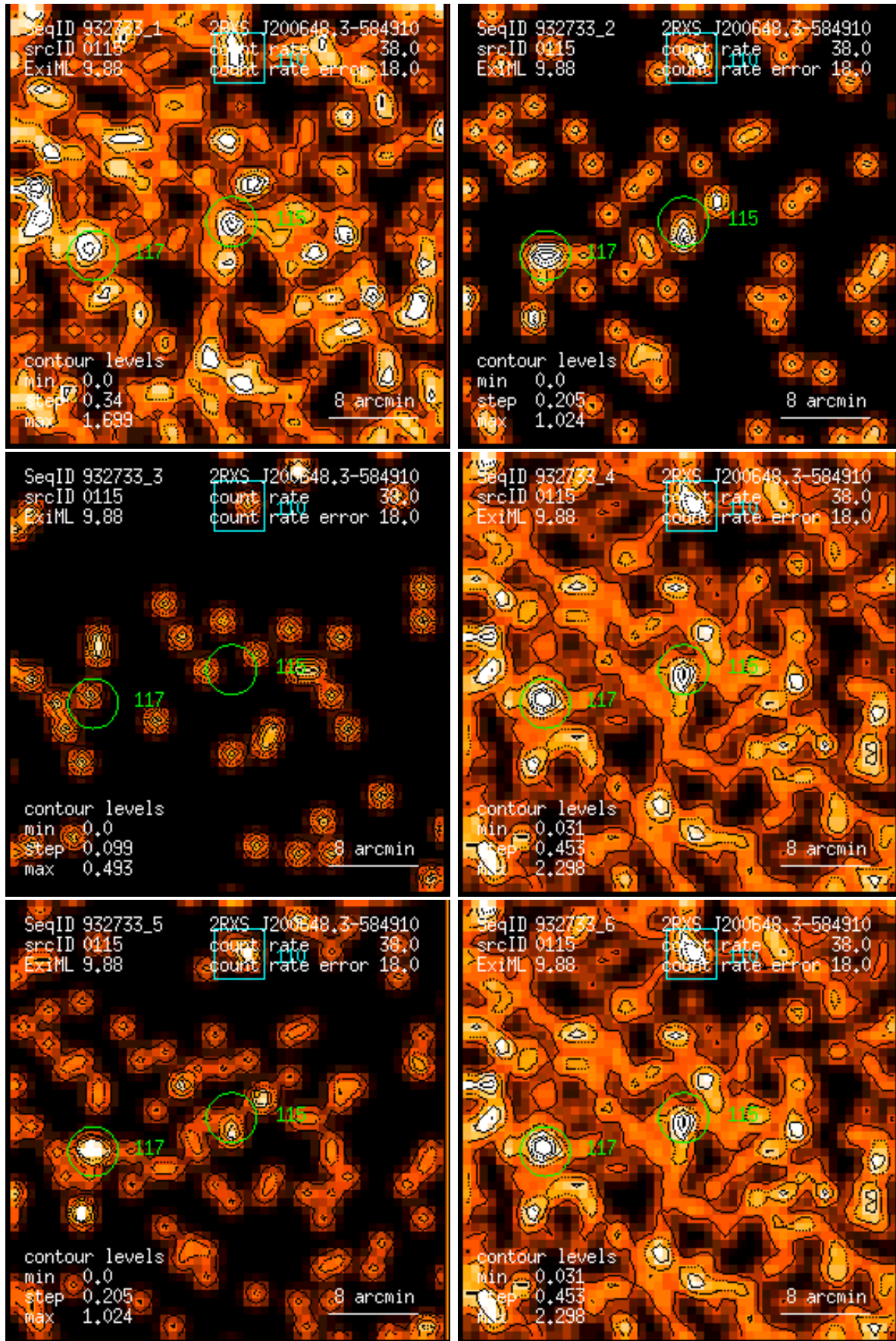
Figure 115: RASS 932733: detection 0115: band rate images, Gaussian filter: (1) PSPC channels 11 – 41, (2) 52 – 90, (3) 91 – 201, (4) 11 – 235, (5) 52 – 201, (6) 11 – 201. Broad band rates in counts/ks. Band rate contour levels in counts/ks/arcmin 2 .
