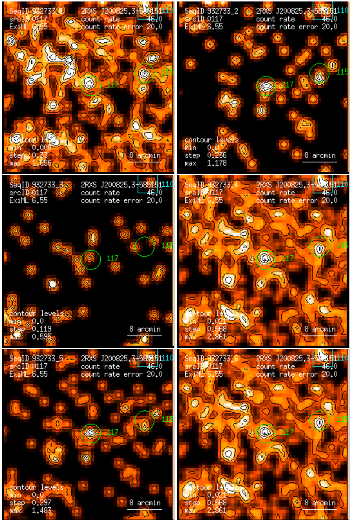
Figure 117: RASS 932733: detection 0117: band rate images, Gaussian filter: (1) PSPC channels 11 – 41, (2) 52 – 90, (3) 91 – 201, (4) 11 – 235, (5) 52 – 201, (6) 11 – 201. Broad band rates in counts/ks. Band rate contour levels in counts/ks/arcmin 2 .
