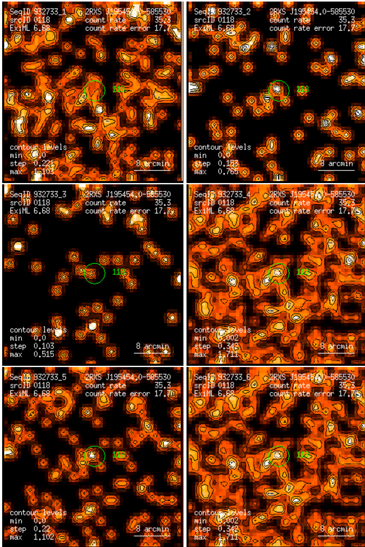
Figure 118: RASS 932733: detection 0118: band rate images, Gaussian filter: (1) PSPC channels 11 – 41, (2) 52 – 90, (3) 91 – 201, (4) 11 – 235, (5) 52 – 201, (6) 11 – 201. Broad band rates in counts/ks. Band rate contour levels in counts/ks/arcmin 2 .
