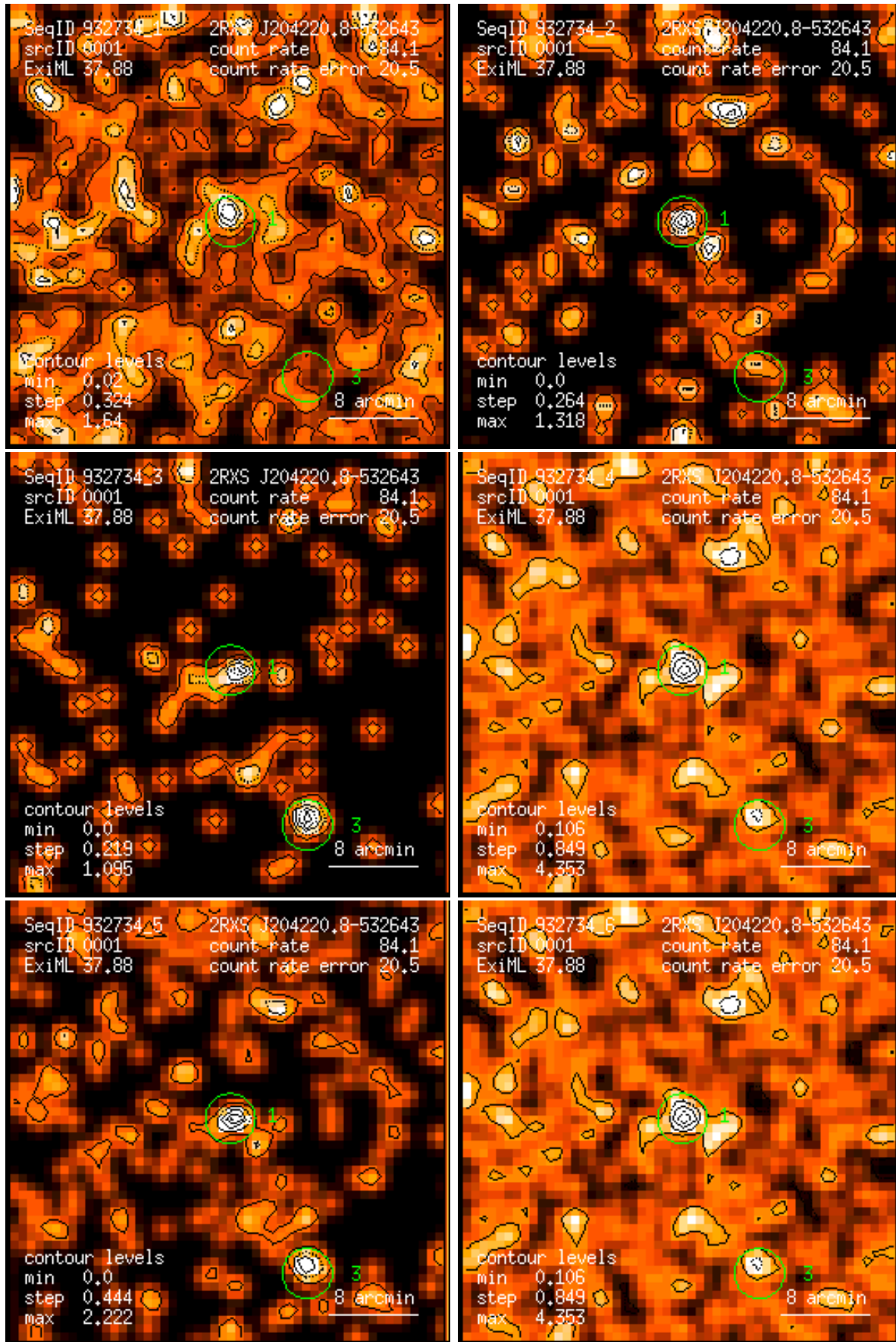
Figure 1: RASS 932734: detection 0001: band rate images, Gaussian filter: (1) PSPC channels 11 – 41, (2) 52 – 90, (3) 91 – 201, (4) 11 – 235, (5) 52 – 201, (6) 11 – 201. Broad band rates in counts/ks. Band rate contour levels in counts/ks/arcmin 2 .
