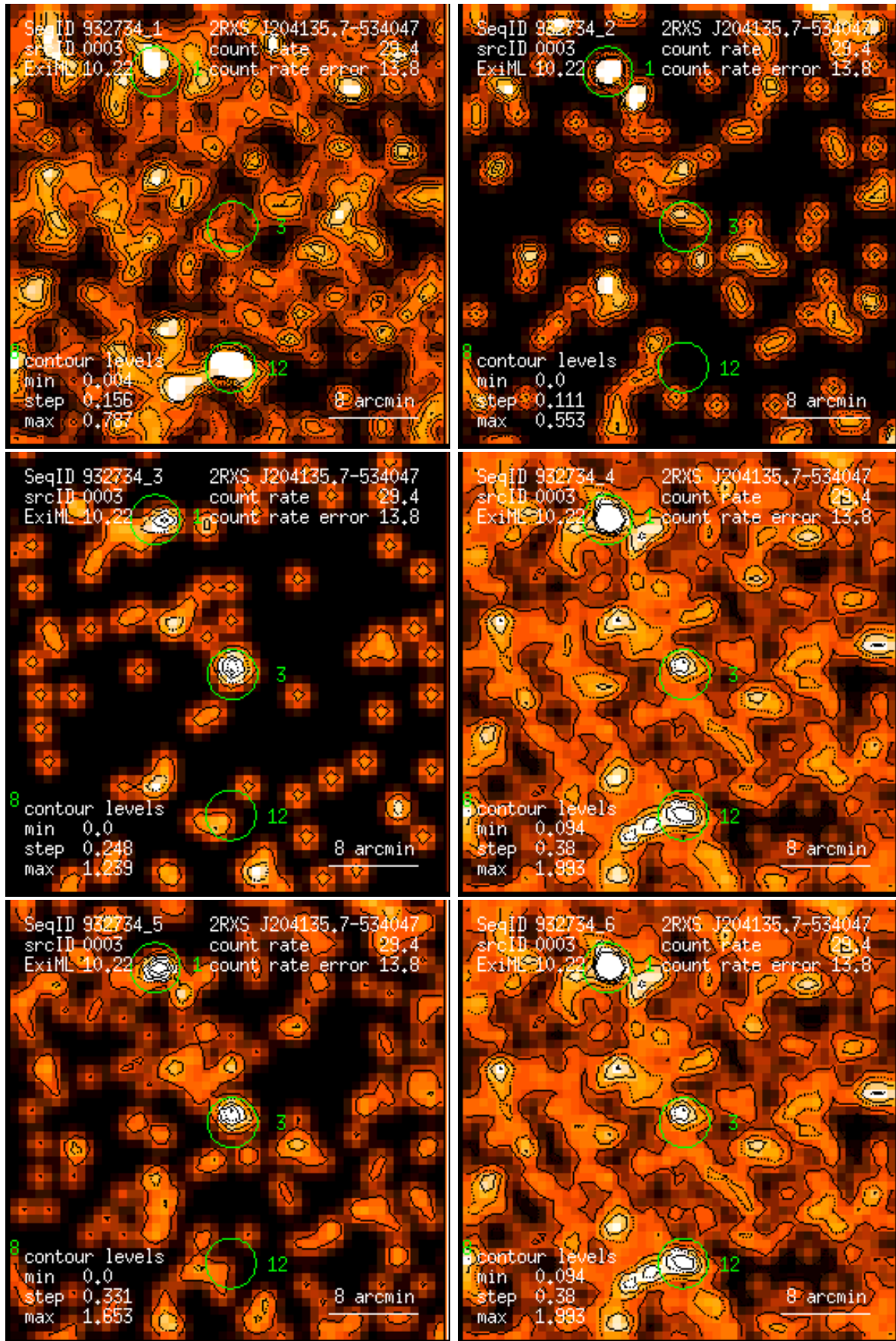
Figure 3: RASS 932734: detection 0003: band rate images, Gaussian filter: (1) PSPC channels 11 – 41, (2) 52 – 90, (3) 91 – 201, (4) 11 – 235, (5) 52 – 201, (6) 11 – 201. Broad band rates in counts/ks. Band rate contour levels in counts/ks/arcmin 2 .
