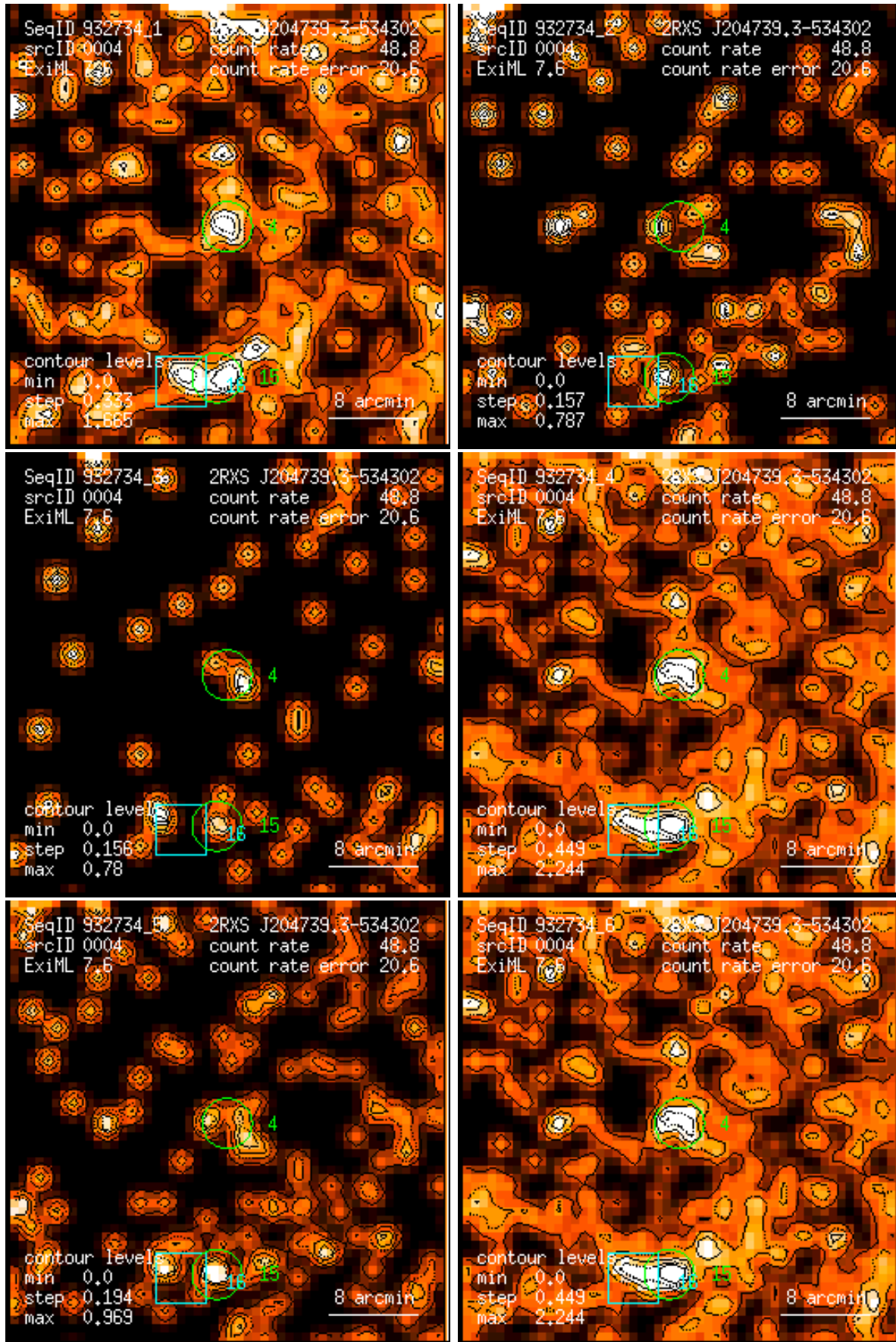
Figure 4: RASS 932734: detection 0004: band rate images, Gaussian filter: (1) PSPC channels 11 – 41, (2) 52 – 90, (3) 91 – 201, (4) 11 – 235, (5) 52 – 201, (6) 11 – 201. Broad band rates in counts/ks. Band rate contour levels in counts/ks/arcmin 2 .
