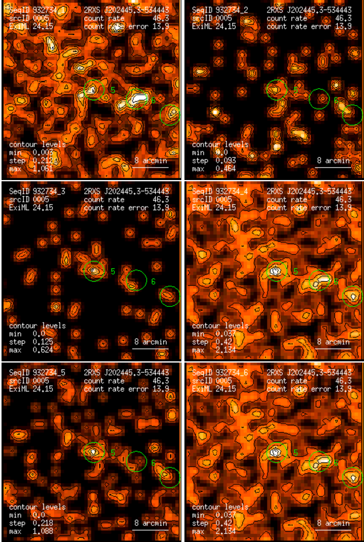
Figure 5: RASS 932734: detection 0005: band rate images, Gaussian filter: (1) PSPC channels 11 – 41, (2) 52 – 90, (3) 91 – 201, (4) 11 – 235, (5) 52 – 201, (6) 11 – 201. Broad band rates in counts/ks. Band rate contour levels in counts/ks/arcmin 2 .
