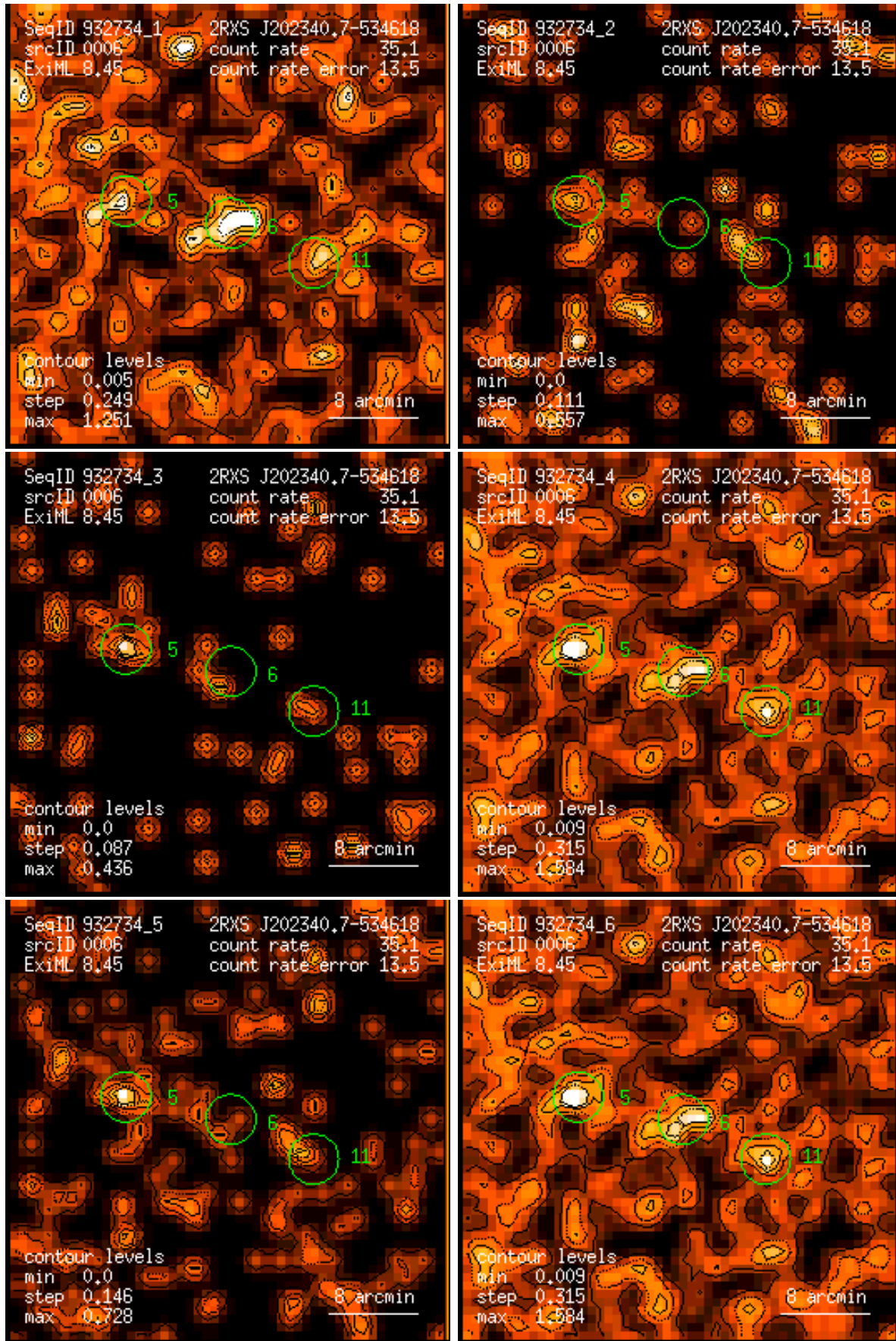
Figure 6: RASS 932734: detection 0006: band rate images, Gaussian filter: (1) PSPC channels 11 – 41, (2) 52 – 90, (3) 91 – 201, (4) 11 – 235, (5) 52 – 201, (6) 11 – 201. Broad band rates in counts/ks. Band rate contour levels in counts/ks/arcmin 2 .
