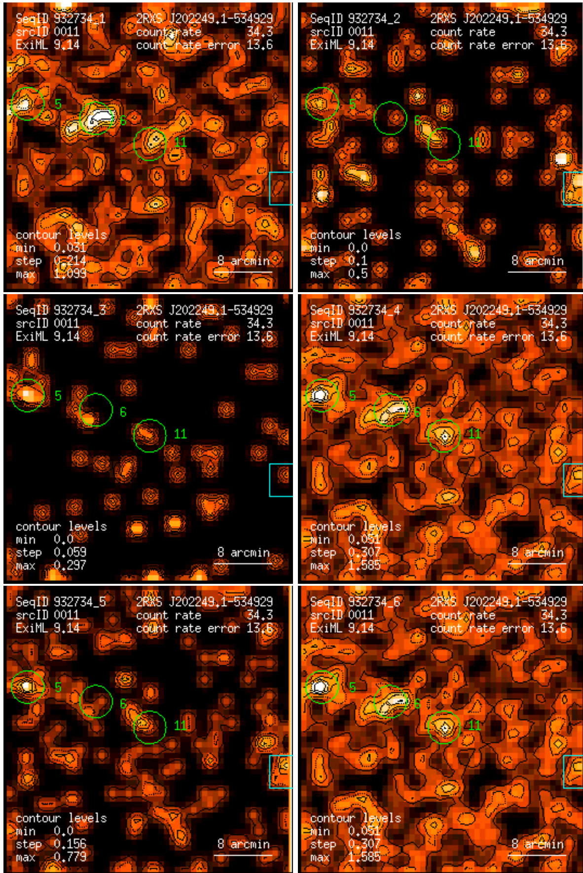
Figure 11: RASS 932734: detection 0011: band rate images, Gaussian filter: (1) PSPC channels 11 – 41, (2) 52 – 90, (3) 91 – 201, (4) 11 – 235, (5) 52 – 201, (6) 11 – 201. Broad band rates in counts/ks. Band rate contour levels in counts/ks/arcmin 2 .
