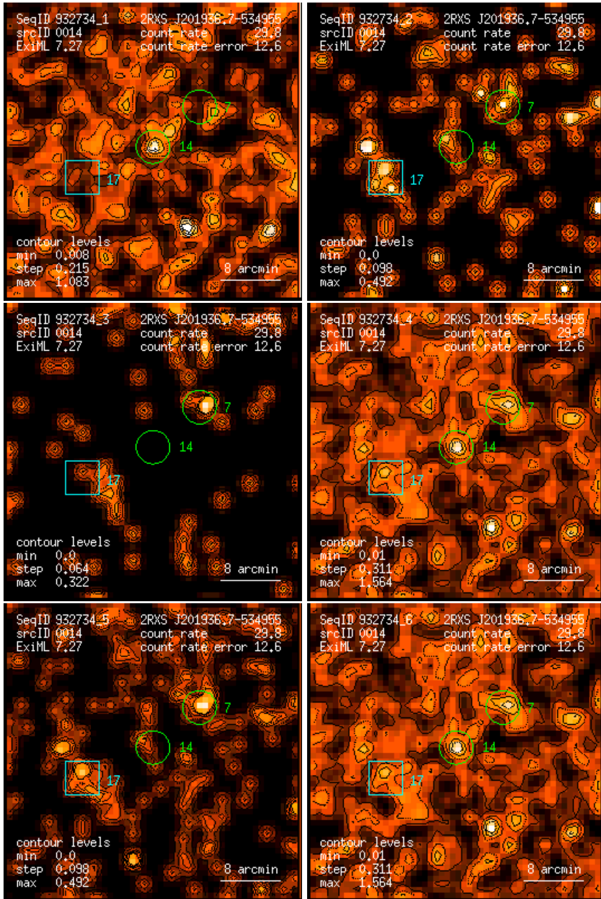
Figure 14: RASS 932734: detection 0014: band rate images, Gaussian filter: (1) PSPC channels 11 – 41, (2) 52 – 90, (3) 91 – 201, (4) 11 – 235, (5) 52 – 201, (6) 11 – 201. Broad band rates in counts/ks. Band rate contour levels in counts/ks/arcmin 2 .
