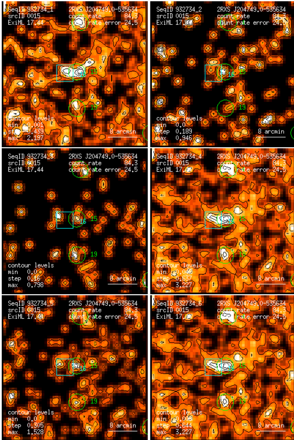
Figure 15: RASS 932734: detection 0015: band rate images, Gaussian filter: (1) PSPC channels 11 – 41, (2) 52 – 90, (3) 91 – 201, (4) 11 – 235, (5) 52 – 201, (6) 11 – 201. Broad band rates in counts/ks. Band rate contour levels in counts/ks/arcmin 2 .
