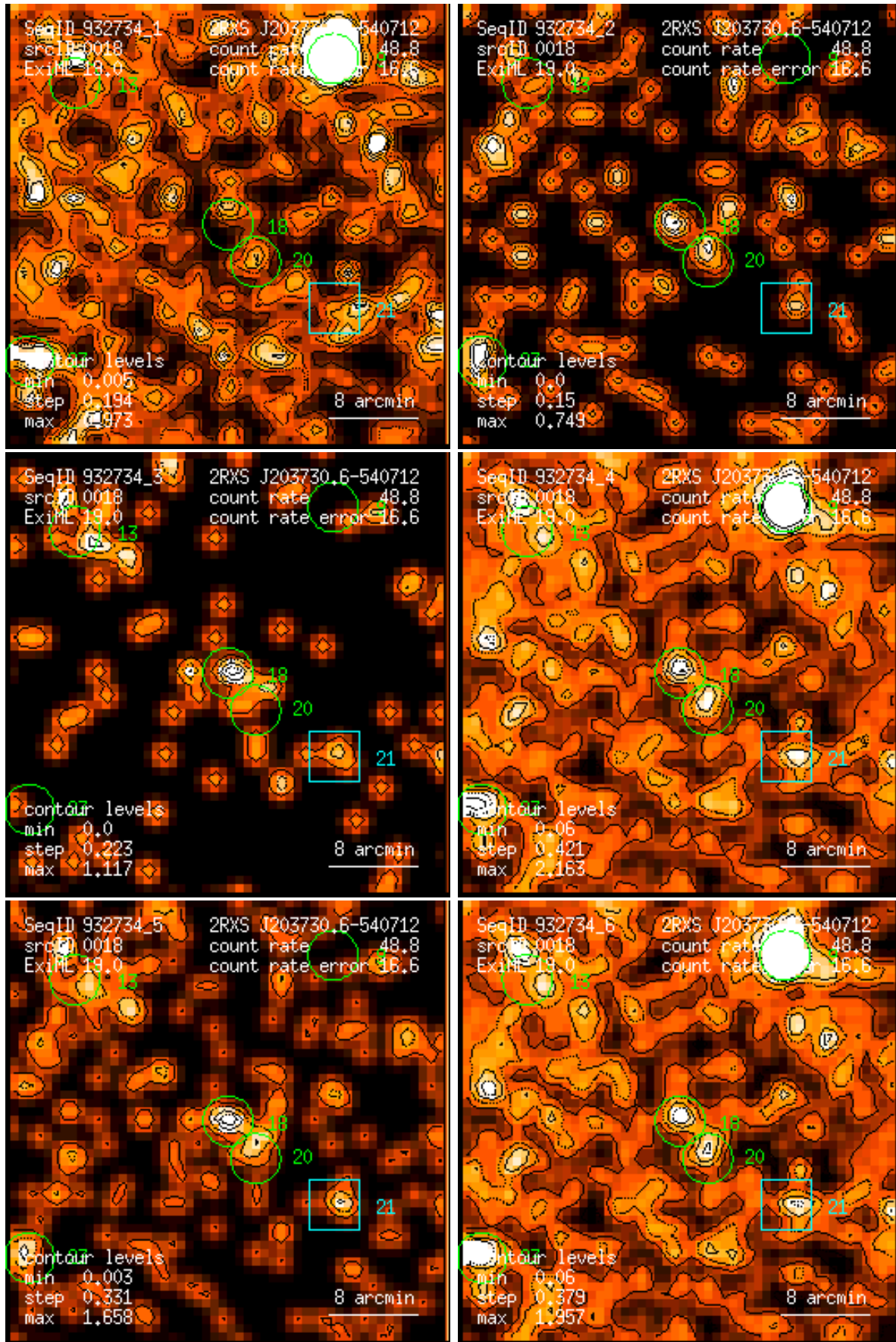
Figure 18: RASS 932734: detection 0018: band rate images, Gaussian filter: (1) PSPC channels 11 – 41, (2) 52 – 90, (3) 91 – 201, (4) 11 – 235, (5) 52 – 201, (6) 11 – 201. Broad band rates in counts/ks. Band rate contour levels in counts/ks/arcmin 2 .
