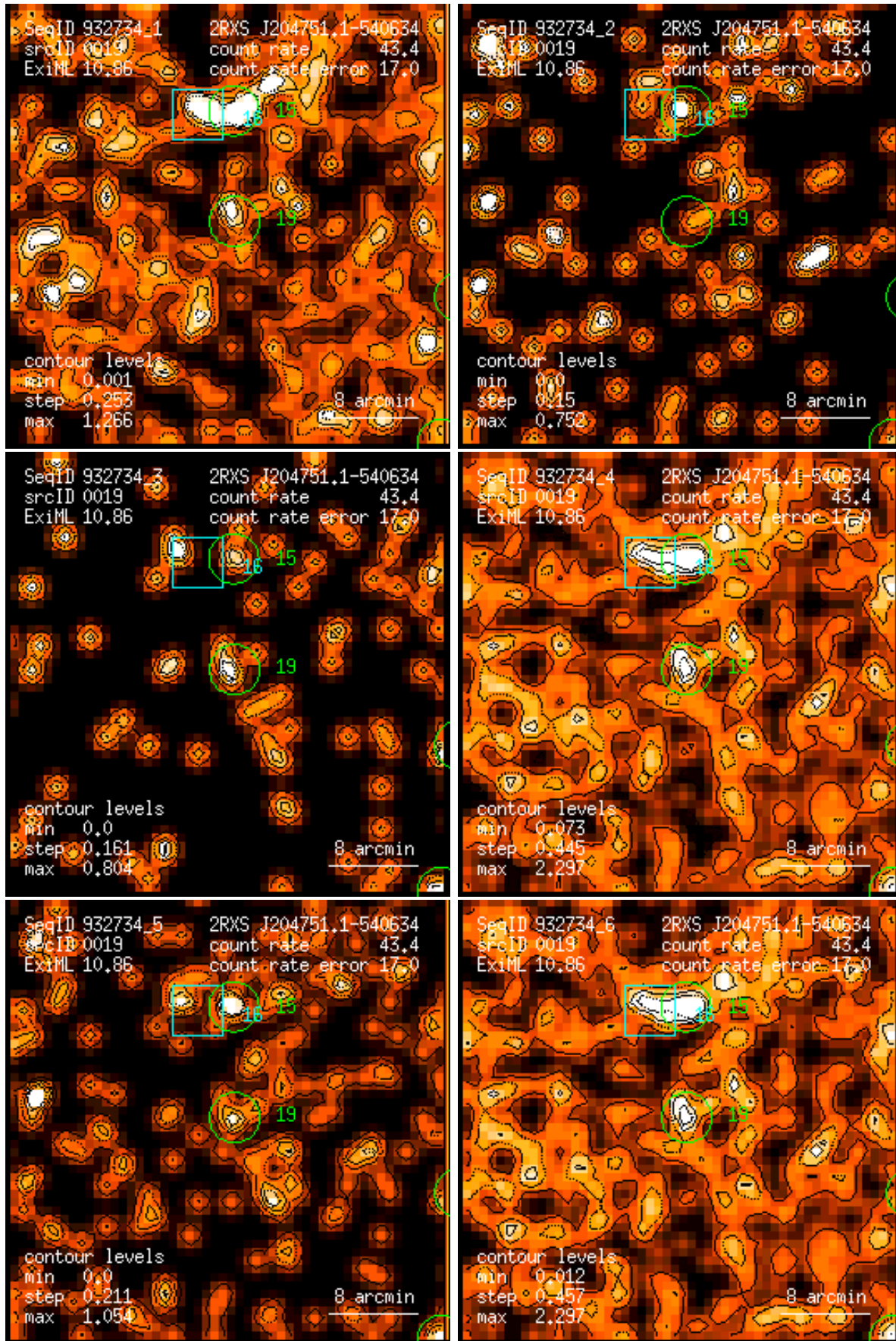
Figure 19: RASS 932734: detection 0019: band rate images, Gaussian filter: (1) PSPC channels 11 – 41, (2) 52 – 90, (3) 91 – 201, (4) 11 – 235, (5) 52 – 201, (6) 11 – 201. Broad band rates in counts/ks. Band rate contour levels in counts/ks/arcmin 2 .
